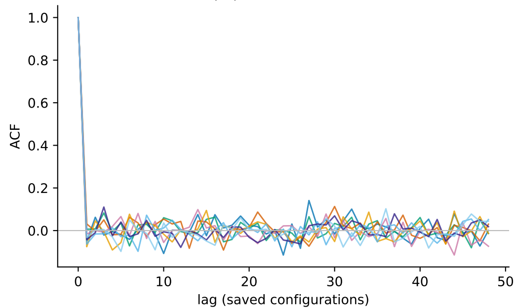
|m| autocorrelation
