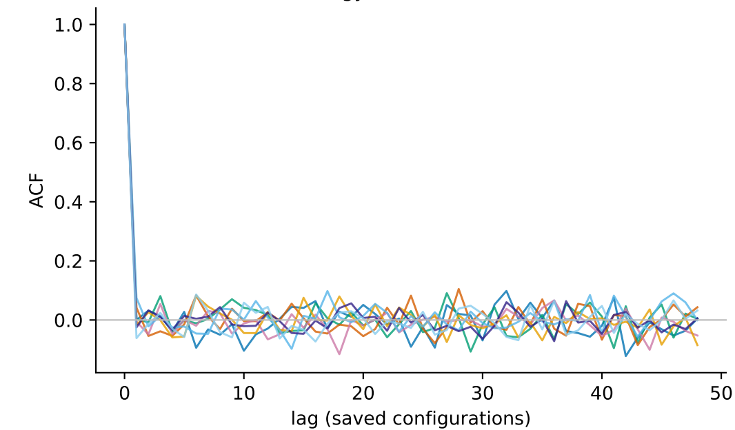
Energy autocorrelation
