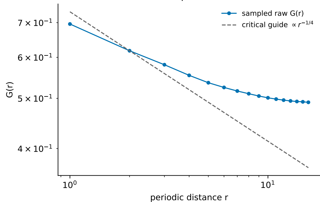
Periodic two-point correlation
