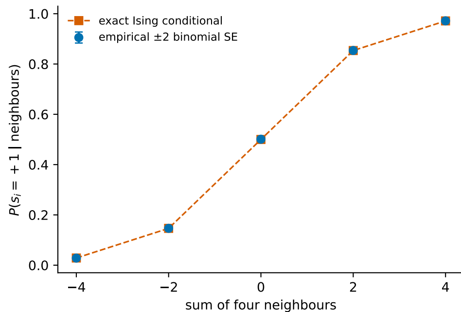
Local Gibbs calibration
