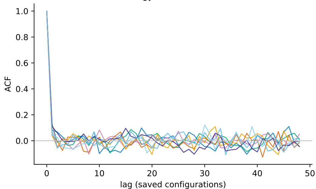
Energy autocorrelation
