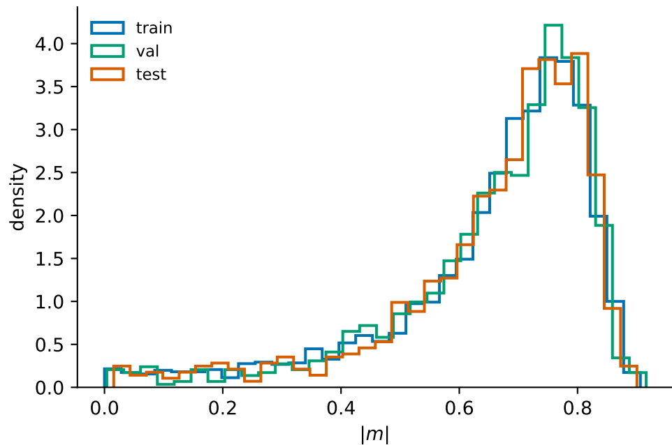
Split consistency: |m|
