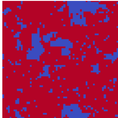
MC reference m=+0.60
