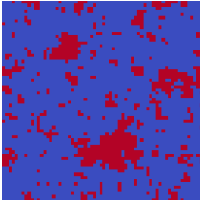
MC reference m=-0.63
