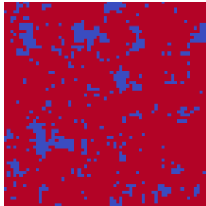
MC reference m=+0.73
