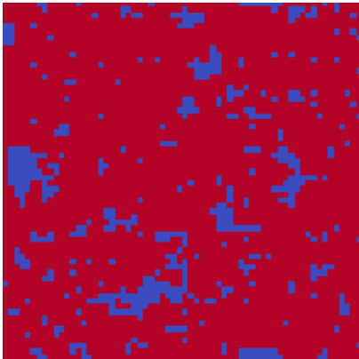
MC reference m=+0.75
