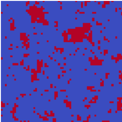
MC reference m=-0.69
