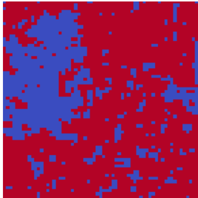
MC reference m=+0.41
