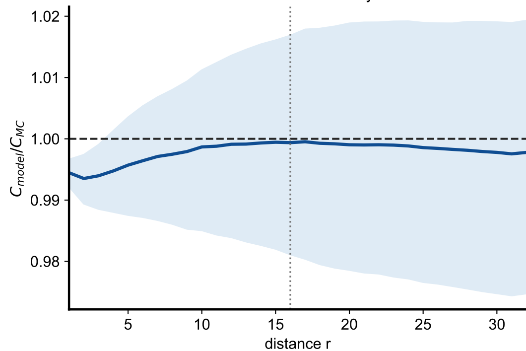
B Correlation fidelity
