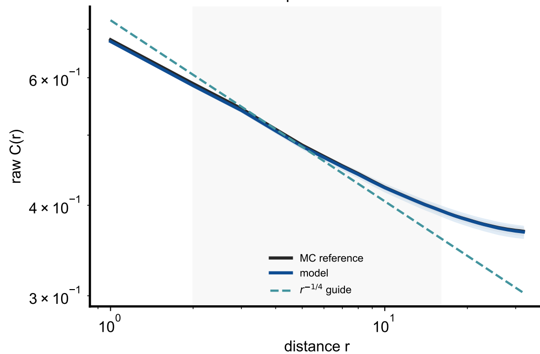
A Two-point correlation
