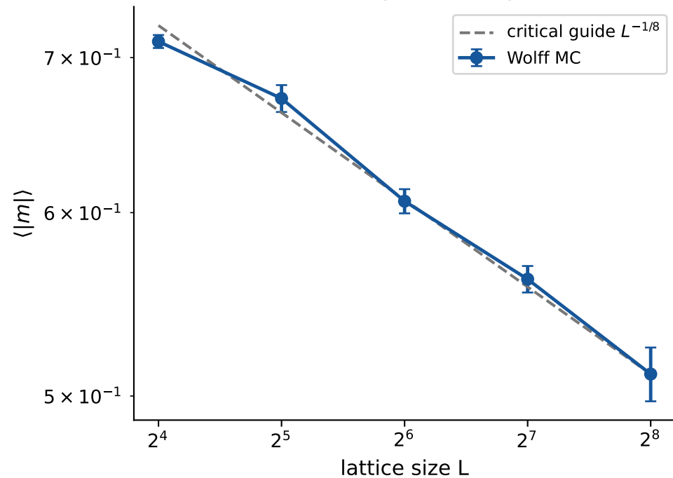
Finite-size scaling: fitted slope -0.121
