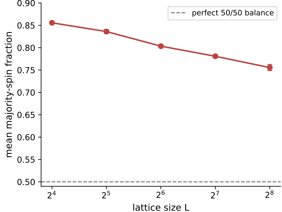
A typical finite critical image is not 50/50
