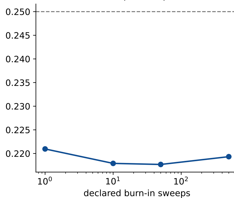
Correlation exponent \hat{\eta} , 4 \leq r \leq 32
