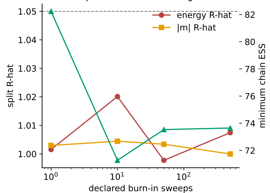
Independent-chain convergence
