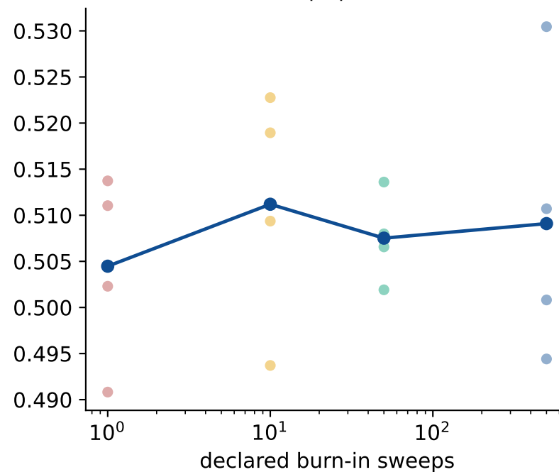
\langle |m| \rangle
