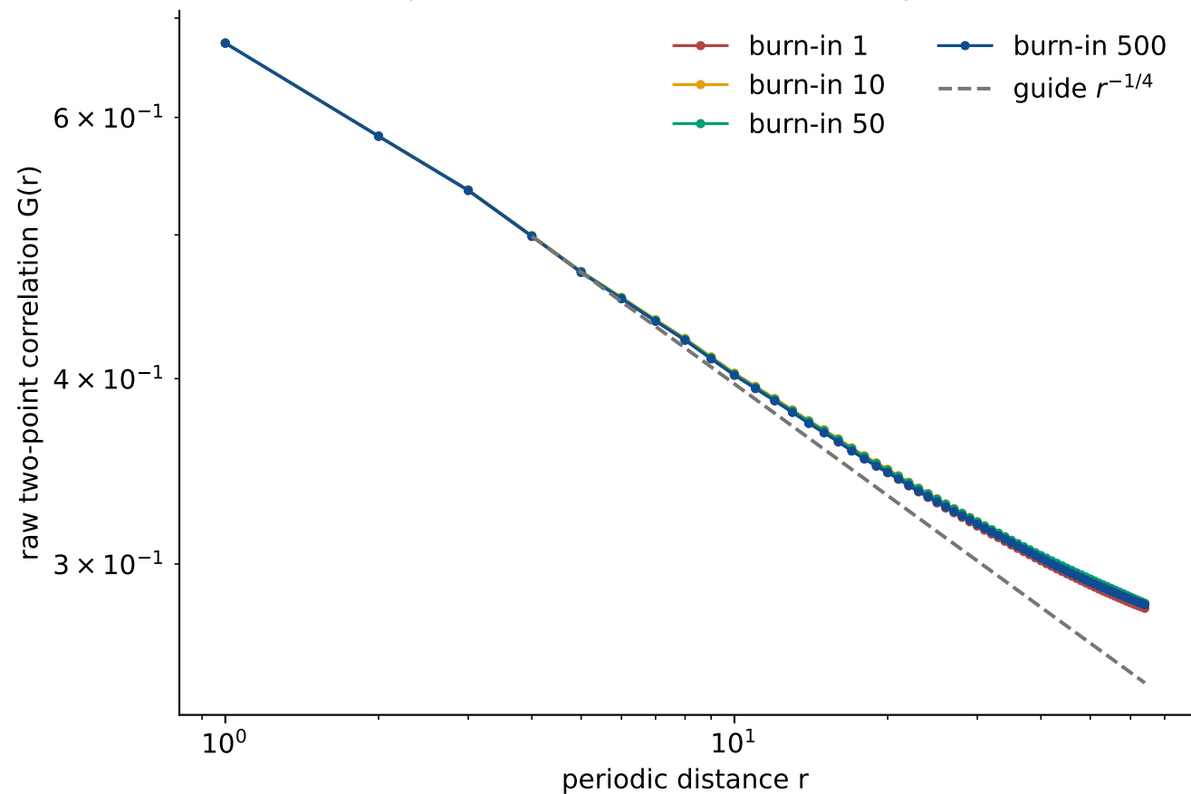
Full periodic L = 256 : burn-in sensitivity of G(r)
