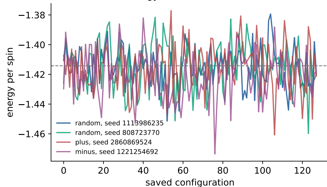
Energy traces, burn-in 500
