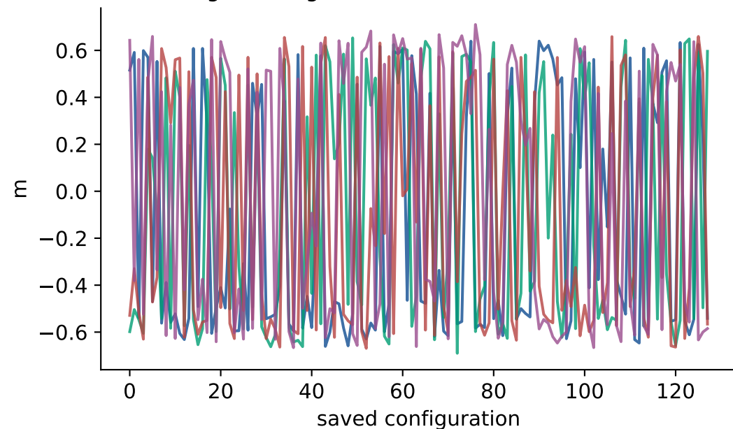
Signed magnetization traces, burn-in 500
