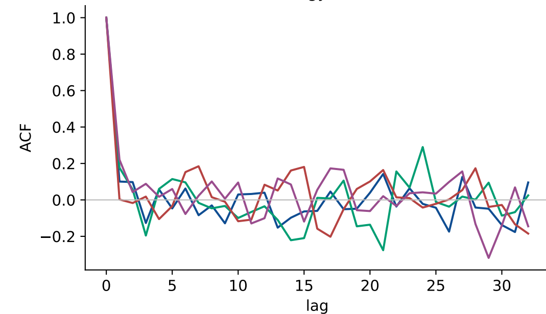
Energy ACF
