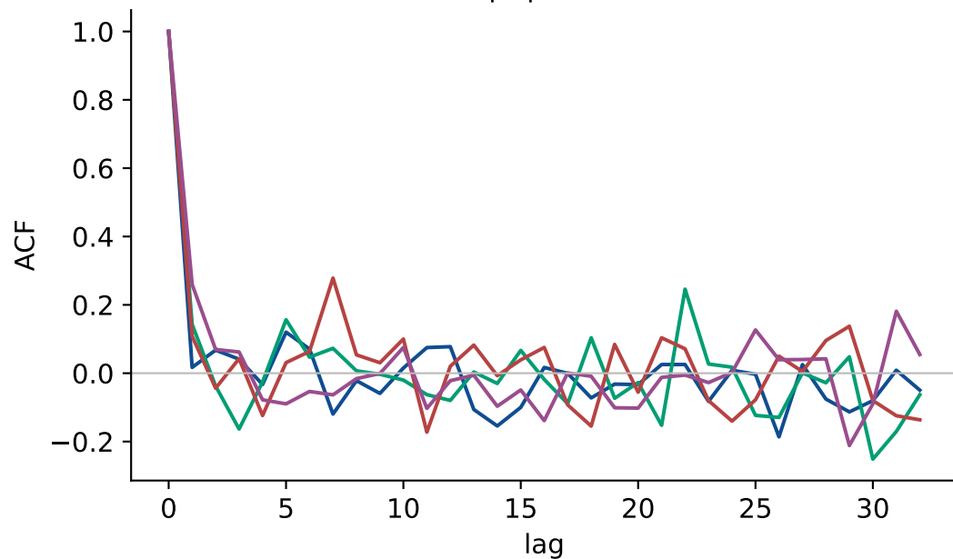
|m| ACF
