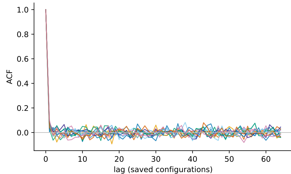
|m| autocorrelation
