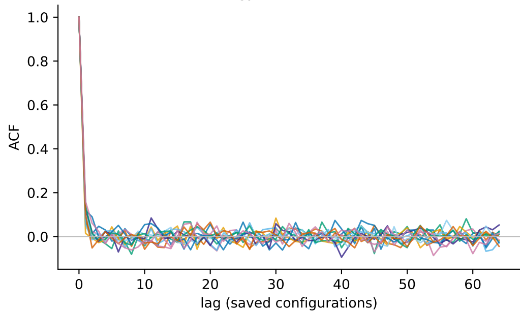
Energy autocorrelation
