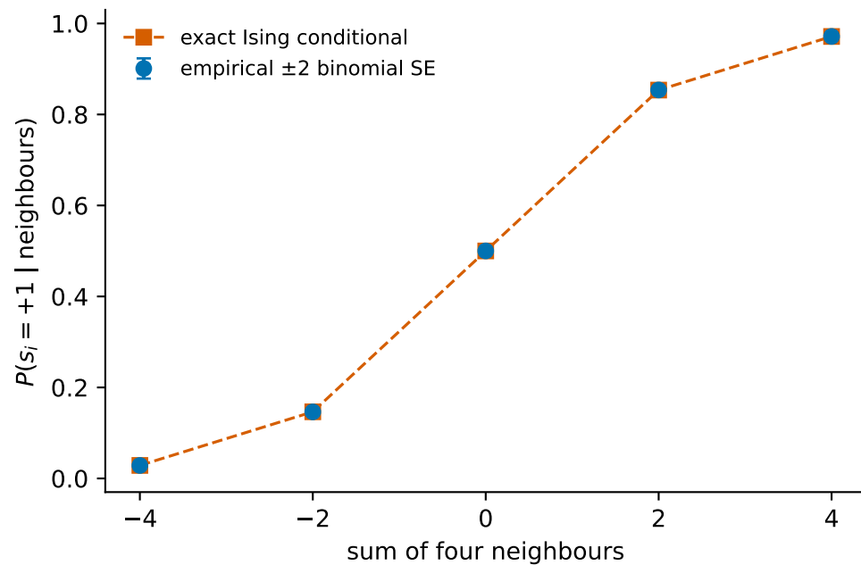
Local Gibbs calibration
