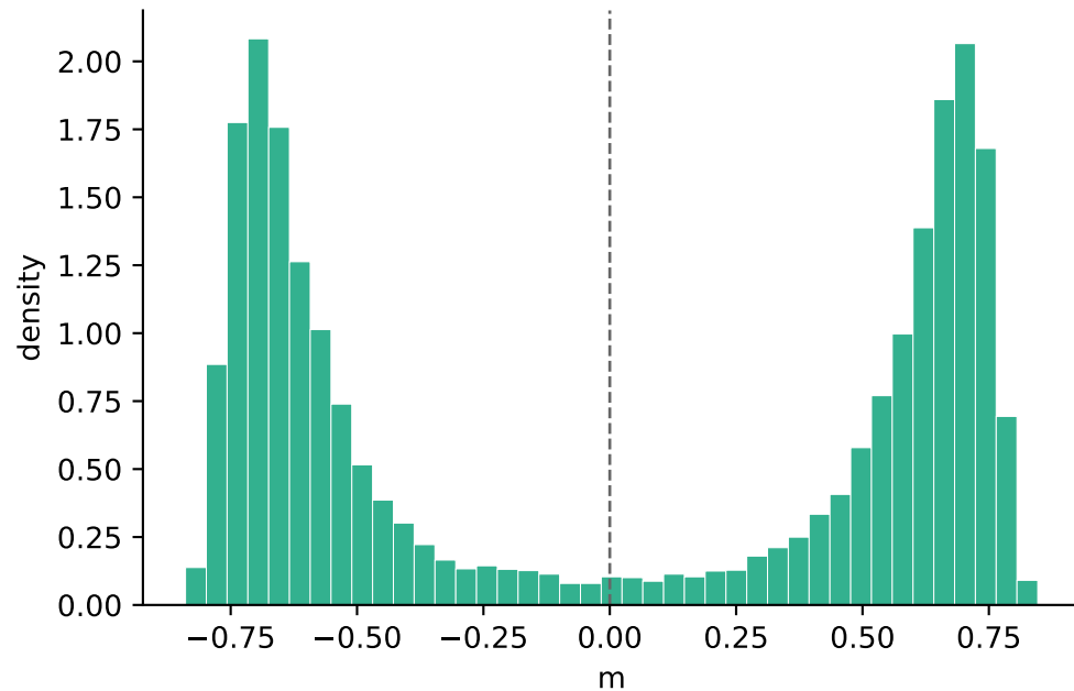
Signed magnetization (spin-flip symmetry)
