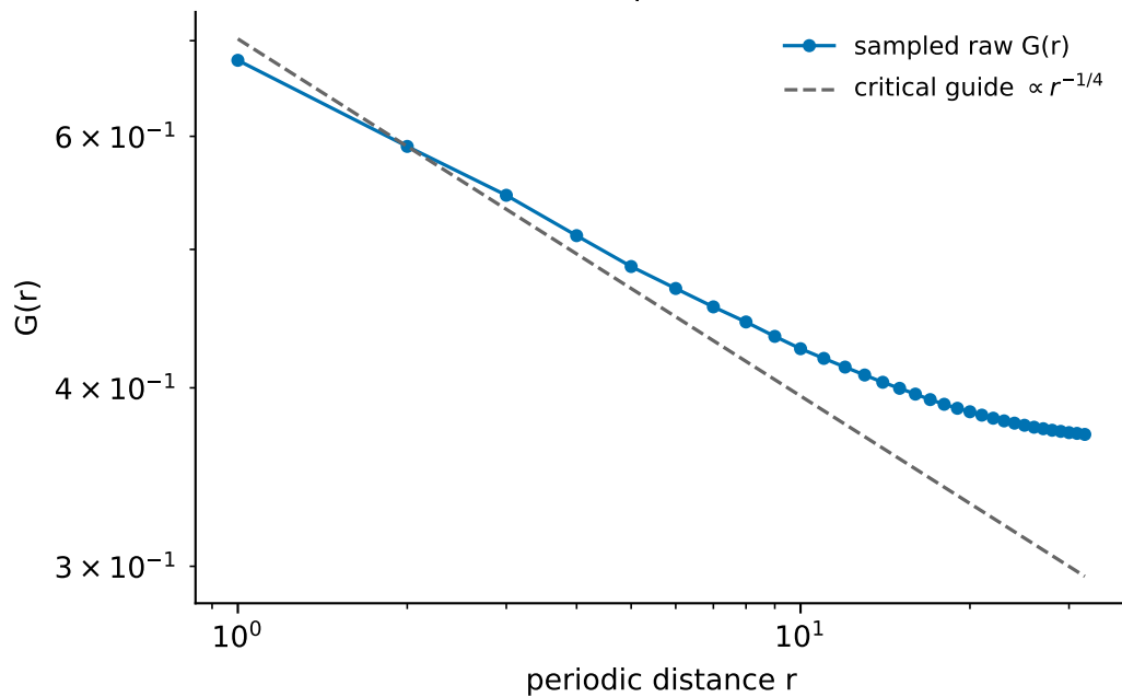
Periodic two-point correlation
