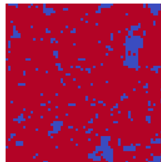
chain 3, saved 1249
