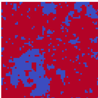
chain 0, saved 1249
