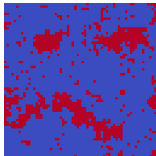
chain 2, saved 1249
