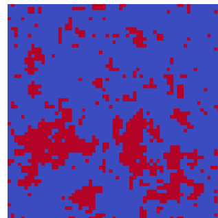
chain 3, saved 416
