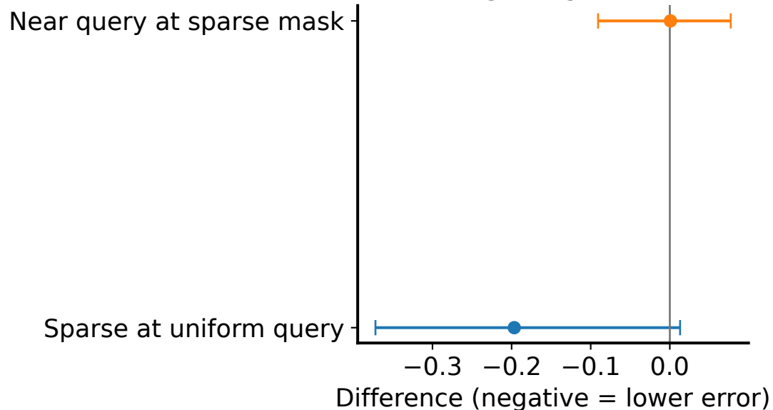
W128 long-range G contrast
