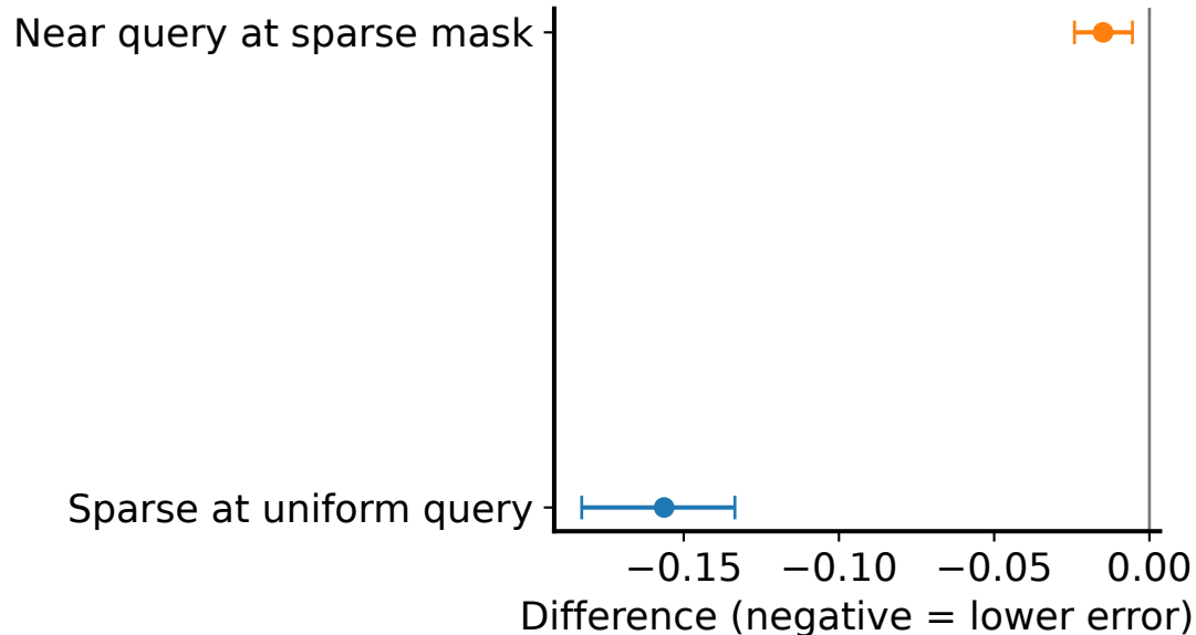
W128 conditional KL contrast
