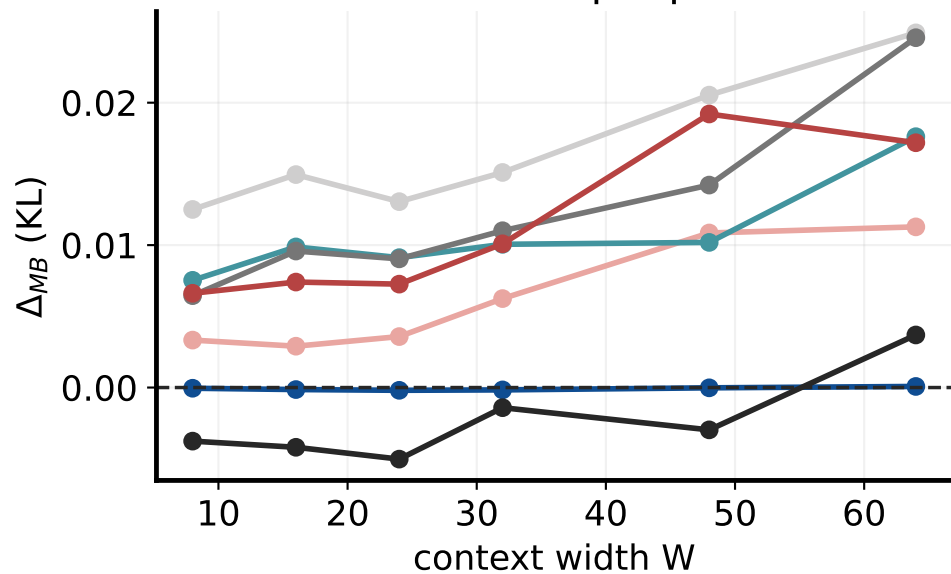
Distant visible-spin pollution
