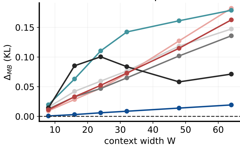
Distant MASK pollution
