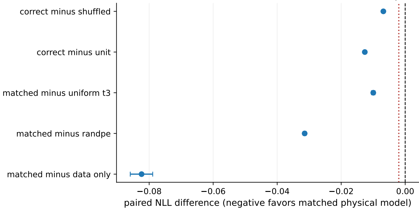
Paired causal contrasts on held-out {3,6} RandomGap
