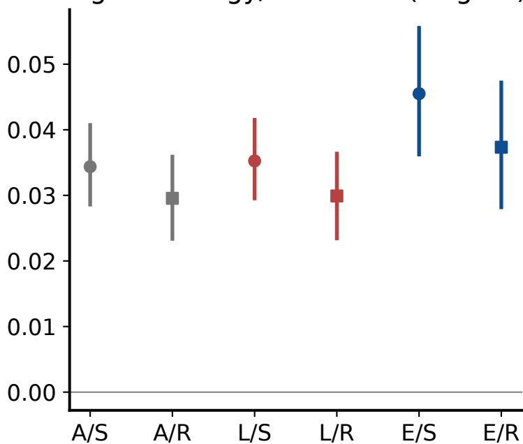
Signed energy/bond bias (target0)
