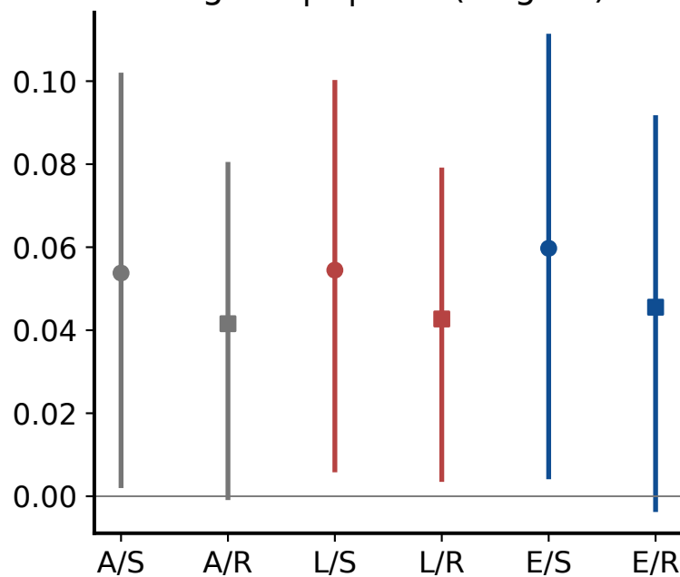
Signed |m| bias (target0)
