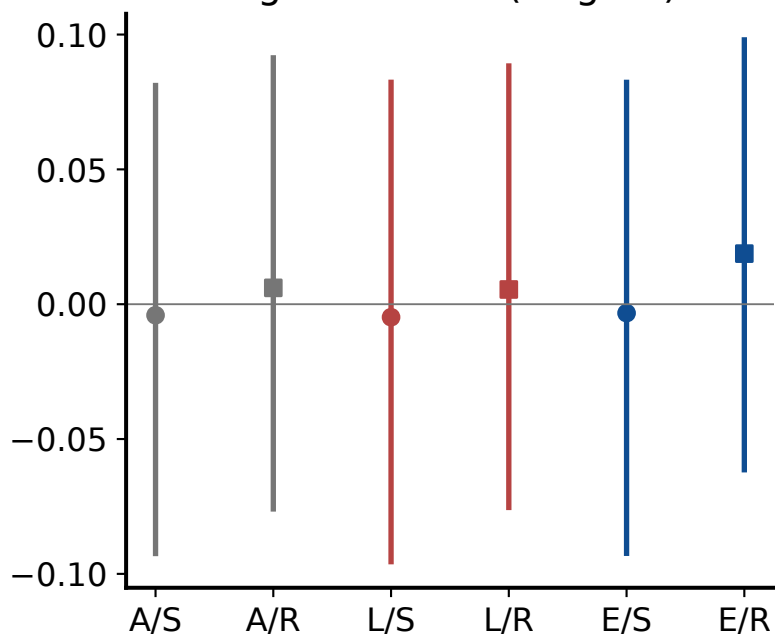
Signed m bias (target0)
