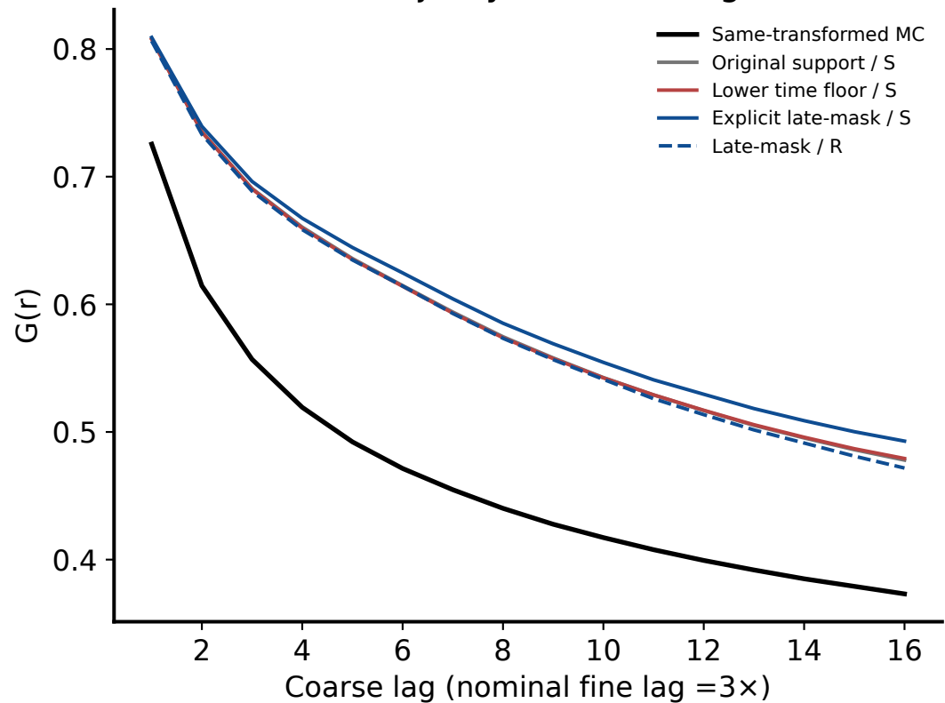
3×3 majority: own MC target
