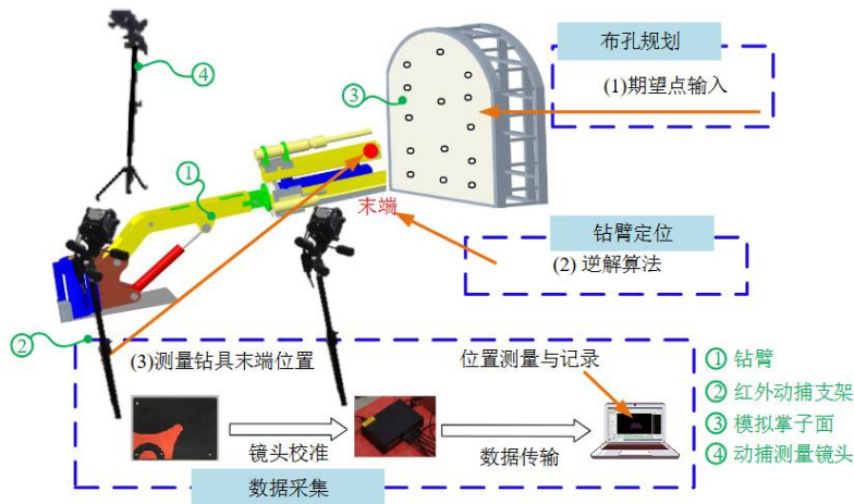
图 4-16 试验数据获取系统 Figure 4-16 Test data acquisition system
