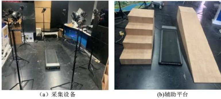
图 2-6 数据采集设备 Fig.2-6 Data acquisition equipment
