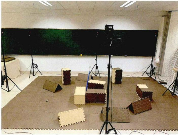
图 2-3 镜头排布方式和飞行实验场景 Fig.2-3 Camera arrangement and flight experiment scene
