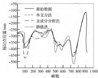
图 4 连续丢失 500 帧的数据修复结果 Fig. 4 Consecutive lost 500 frames of data restoration results
