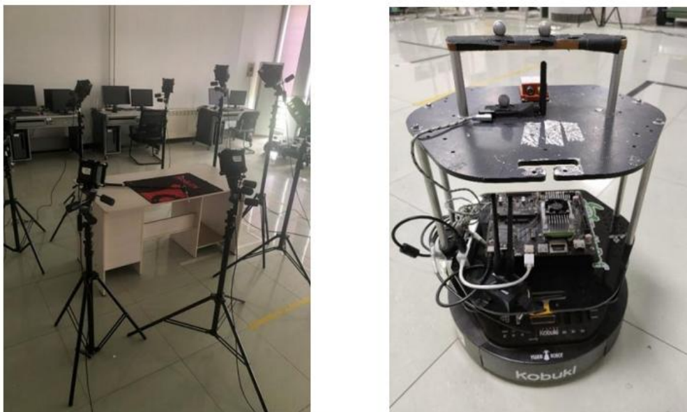
图 4-4 视觉捕捉设备及机器人平台 Figure 4-4 Vision capture equipment and robot platform
