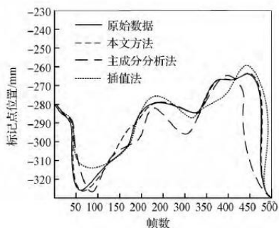
图 3 连续丢失 100 帧的数据修复结果 Fig. 3 Consecutive lost 100 frames of data restoration results
