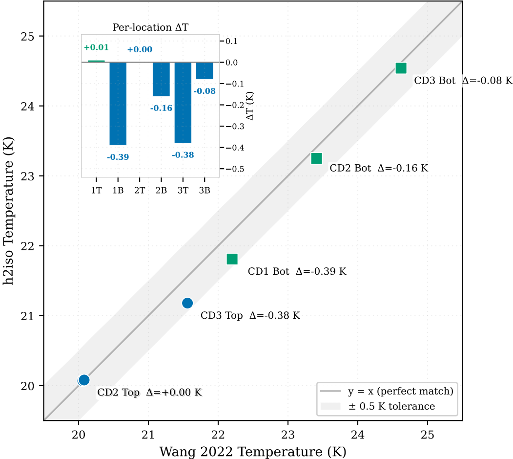
ISS-O Three-Column Temperature Validation (CD1+CD2+CD3 vs Wang 2022)
