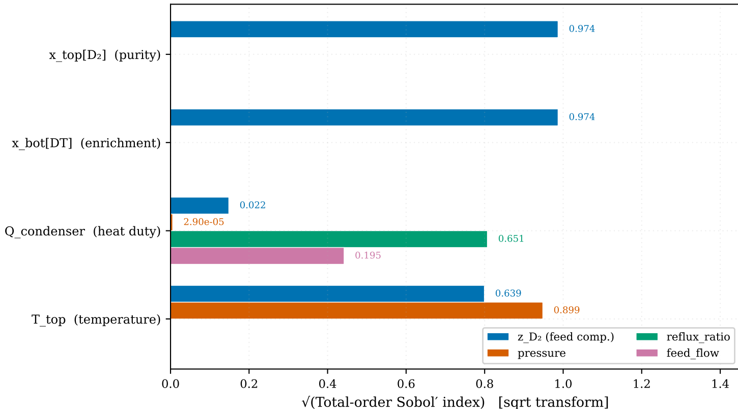
CD2 Column: Global Sensitivity Analysis (Sobol' Indices) UQ over z_{D_2} , pressure, reflux ratio, feed flow (N=32 base, 192 samples)
