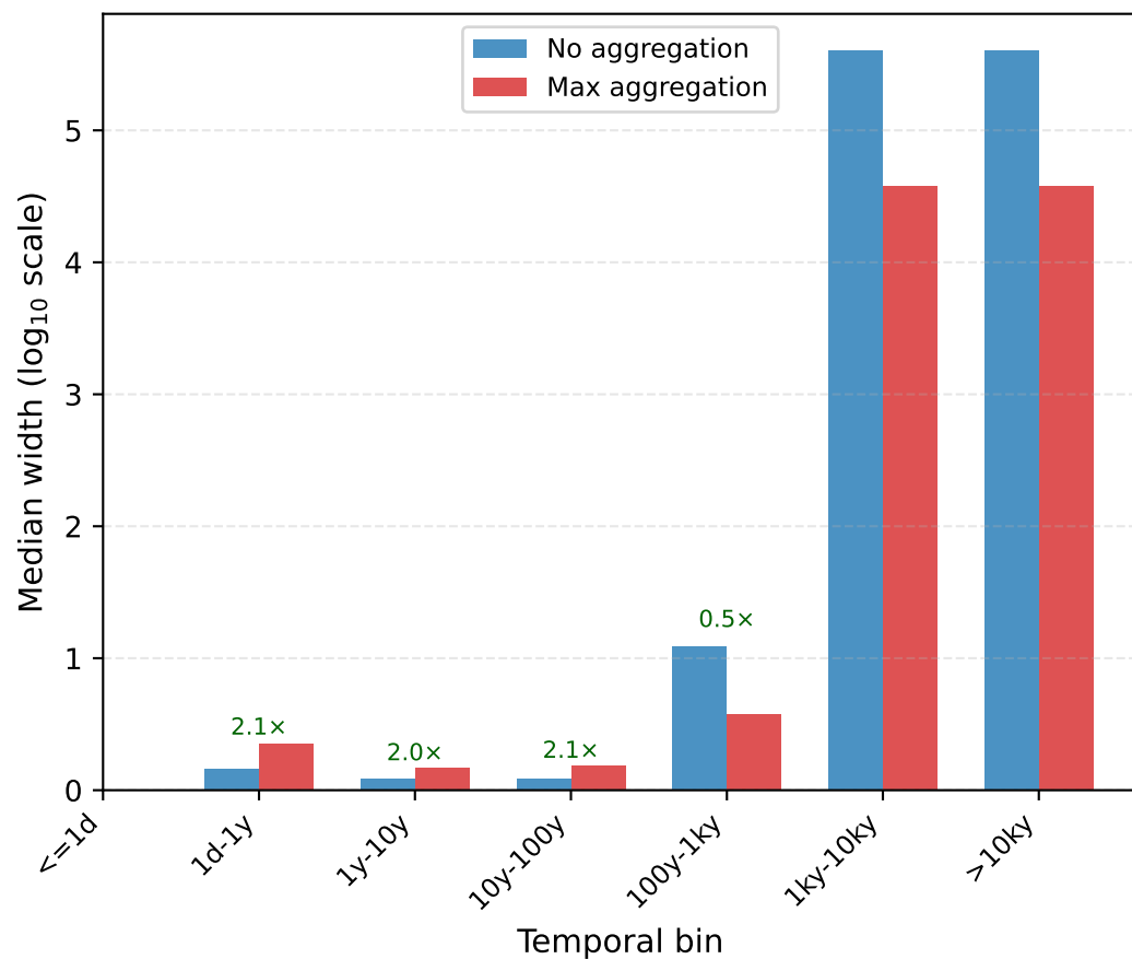
Atoms H3
