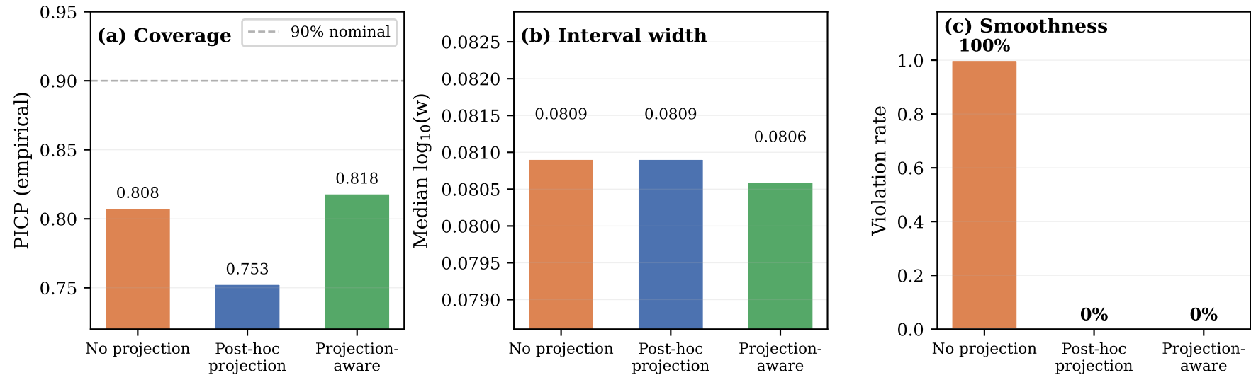
Projection-strategy ablation ( ^3\text{H} , D_{224} , CV+)
