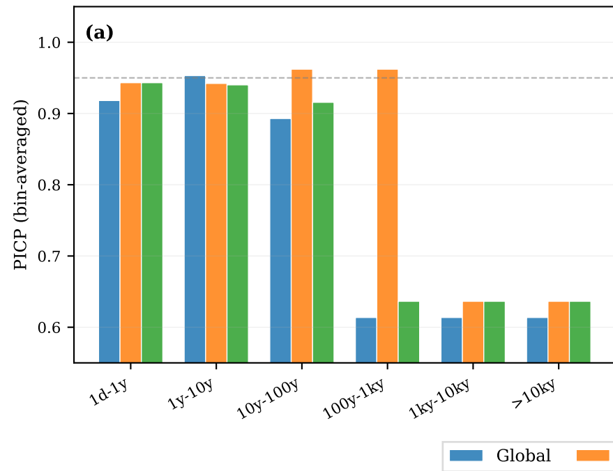
Coverage by time bin
