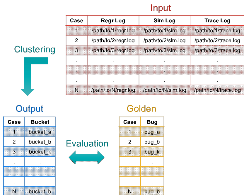
Fig. 2: Problem formulation: input table and output table.
