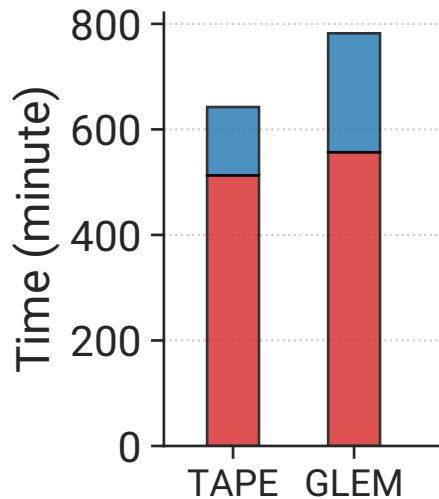
(c) Ogbn-arxiv
