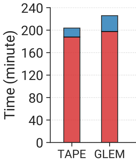
(b) Pubmed
