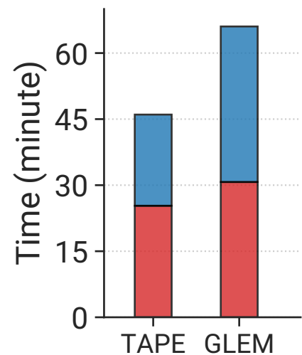
(a) Ogbn-products
