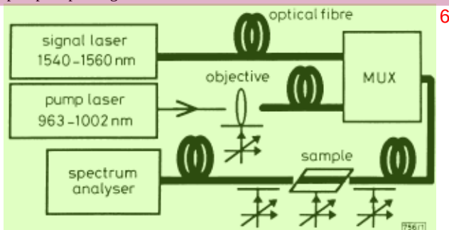
Fig. 1 Schematic diagram of gain and noise factor measurements setup
