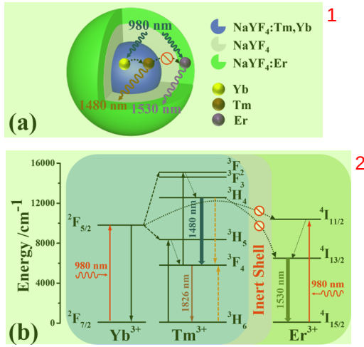
Fig. 1. (a) Structure diagram of core-multishell NPs and (b) energy level diagrams of \text{Tm}^{3+} , \text{Yb}^{3+} , and \text{Er}^{3+} ions, and possible downconversion processes under 980-nm laser excitation.
