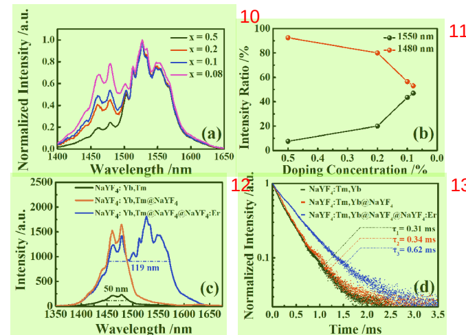
Fig. 2. \text{NaYF}_4\text{:Tm,Yb@NaYF}_4\text{@NaYF}_4\text{:x%Er} NPs: (a) emission spectra and (b) intensity ratios of 1.48- \mu\text{m} and 1.53- \mu\text{m} emissions; \text{NaYF}_4\text{:Tm,Yb@NaYF}_4\text{@NaYF}_4\text{:0.08%Er} : (c) emission spectra and (d) decay curves of 1480-nm fluorescence from the {}^3\text{H}_4 level in different growth stages.
