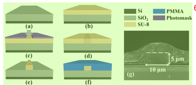
Fig. 3. (a)–(f) Preparation process of the TECDWA and (g) SEM image of the waveguide.
