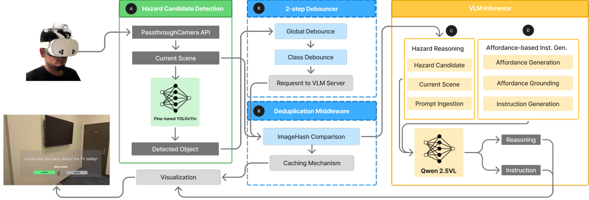
Figure 1: Overview of the proposed framework for real-time hazard inference in XR environments. (a) Candidate hazard objects are first detected using a fine-tuned YOLOv11n model running locally on the HMD. When a candidate object is detected, the current scene and detection information are prepared for VLM-based reasoning. (b) Before transmission to the VLM server, two optimization strategies are applied: a two-step debouncing mechanism that reduces redundant server calls, and a deduplication middleware that prevents visually similar frames from being repeatedly processed. (c) The VLM then uses the scene context and detection information to infer whether the detected object represents a potential hazard. (d) If a hazard is confirmed, the system generates an affordance-based safety instruction to guide the user toward an appropriate corrective action.
