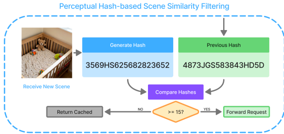
Figure 3: Perceptual hash-based scene deduplication middleware for reducing redundant VLM inference.
