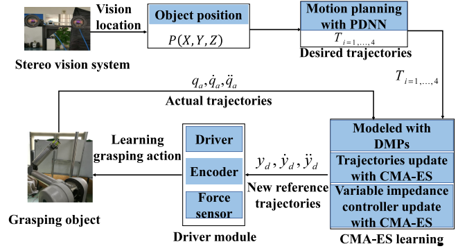
Fig. 6. Learning process of the grasping task.
