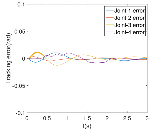
Fig. 18. Tracking error of manipulator.
