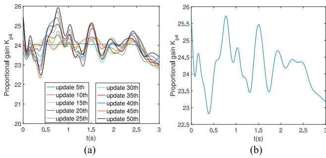
Fig. 15. exp1: Proportional Gain K_{p4} learning results of controller. (a) Learning process of K_{p4} . (b) K_{p4} at the last update.
