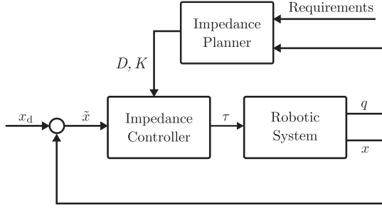
Fig. 3. Proposed algorithm acts by modifying the gains K and D of the impedance controller based on the current state q of the robot and on some performance requirements (explained later on).
