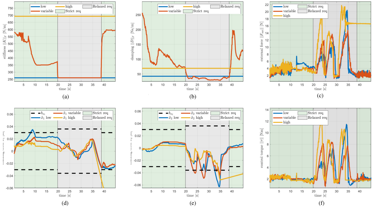
Fig. 11. Experiments with the Franka Emika Panda using the noninertia shaping controller [69]. The impedance gains for the cases of low, high, and variable (Algorithm 1) impedance are shown in (a) and (b). Here, the damping for the fixed impedance cases is computed with the critically damped condition, as traditionally done. The norm of the contact forces is plotted in (c). For a fair comparison, the fixed gains are the same as in the inertia shaping case. The tracking errors along \hat{x}_1 and \hat{x}_2 together with the boundaries used by the impedance planner are shown in (d) and (e). The norm of the control torque is plotted in (f). (a) Frobenius norm of stiffness matrices. (b) Frobenius norm of damping matrices. (c) Norm of external force. (d) Tracking error along \hat{x}_1 . (e) Tracking error along \hat{x}_2 . (f) Norm of control torque.
