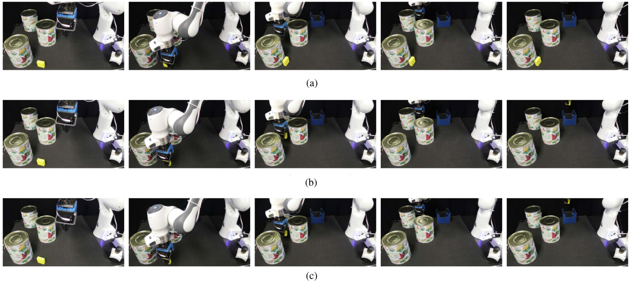
Fig. 8. Experiments using the inertia shaping controller in [10]. Fixed-low impedance reduces precision, causing task failure. Fixed-high gains, instead, produce high external forces. The Standard Method attempts to balance precision with compliance. (a) Low decoupled impedance reduces precision and increases compliance. (b) High decoupled impedance increases precision and reduces compliance. (c) Standard Method alternates high and low impedance.
