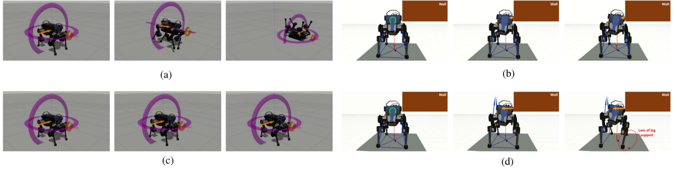
Fig. 2. High impedance versus low impedance on the robot ANYmal with a Cartesian impedance controller regulating its torso. With low impedance, when subject to an external force disturbance, the robot cannot track correctly the reference position and falls. However, more robustness to unforeseen contacts is displayed. High impedance, instead, ensures tracking by rejecting force disturbances, but environment interaction destabilizes the robot, which loses support on two legs (dashed red circle). (a) Constant force disturbance with low impedance. (b) Environment interaction with low impedance. (c) Constant force disturbance with high impedance. (d) Environment interaction with high impedance.
