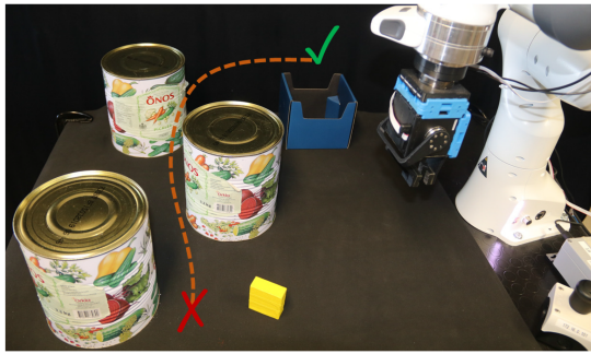
Fig. 7. Experimental setup for the case of nondiagonally dominant inertia. Franka Emika Panda robot mounts an ATI Mini45 force/torque sensor and a QB SoftClaw gripper. The object (■) should be grasped and transported from the initial (×) to the goal (✓) position.
