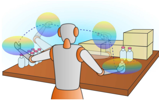
Fig. 1. Planning a variable impedance, based on requirements on tracking and robustness, shapes the impedance ellipsoid and ensures better performance.
