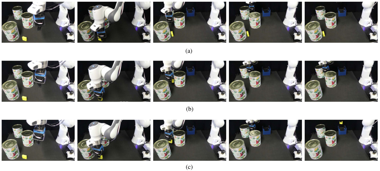
Fig. 9. Experiments using the noninertia shaping controller (similar to [69]). Due to coupling, low gains cause high imprecision and high gains produce external forces that violate the robot safety limits. In both cases, the task fails. Algorithm 1 sets the impedance required to properly balance tracking error reduction and impedance minimization. (a) Low coupled impedance reduces precision and increases compliance. (b) High coupled impedance increases precision and reduces compliance. (c) Algorithm 1 varies precision and compliance as required.
