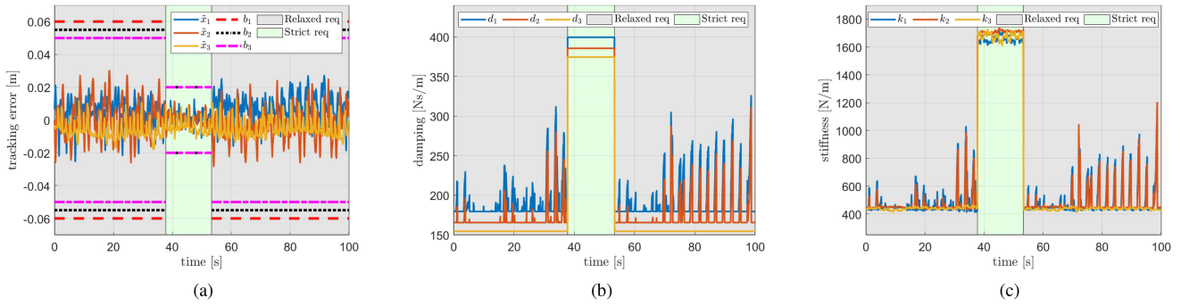
Fig. 6. Experiment with ANYmal on rough terrain. (a) Margins b_i are tightened at t = 38 s and later reset at t = 53 s. The tracking error is always maintained within the boundaries. (b), (c) Algorithm 1 automatically computes impedance gains. (a) Translational tracking error. (b) Translational damping coefficients. (c) Translational stiffness coefficients.
