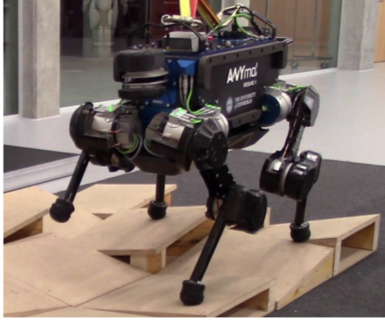
Fig. 5. Experiments on ANYmal. ANYmal engaging rough terrain aided by our impedance planning algorithm.
