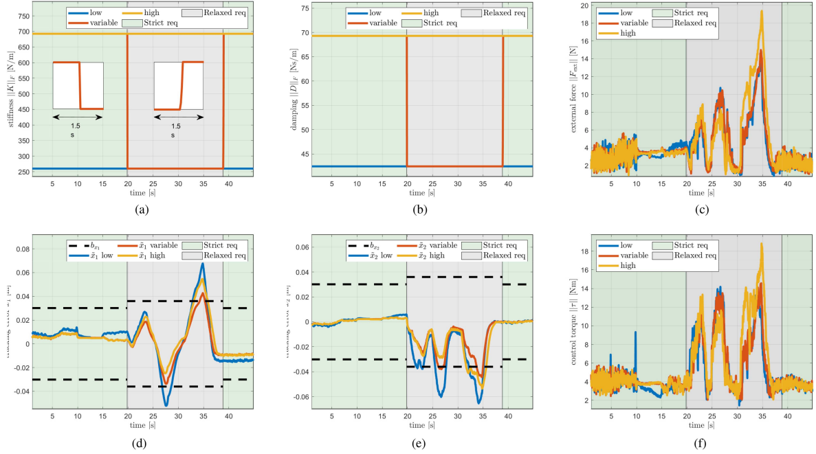
Fig. 10. Experiments with the Franka Emika Panda using the inertia shaping controller [10]. The impedance gains for the cases of low, high, and variable ( Standard Method ) impedance are shown in (a) and (b). The inserts in (a) show how the Standard Method smooths sudden variations using [12] for guaranteeing stability. The norm of the contact forces is plotted in (c). Notice that in real-world scenarios, the contact forces are not ideally impulsive. The tracking errors along \hat{x}_1 and \hat{x}_2 together with the boundaries used by the impedance planner are shown in (d) and (e). The norm of the control torque is plotted in (f). (a) Frobenius norm of stiffness matrices. (b) Frobenius norm of damping matrices. (c) Norm of external force. (d) Tracking error along \hat{x}_1 . (e) Tracking error along \hat{x}_2 . (f) Norm of control torque.
