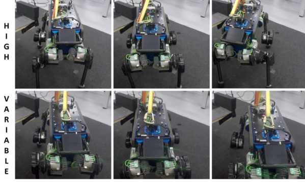
Fig. 4. Experiments on ANYmal. ANYmal colliding with an unperceived obstacle. A fixed high impedance produces high contact forces that trigger the emergency stop. Variable impedance, instead, increases robot compliance to withstand the disturbance.
