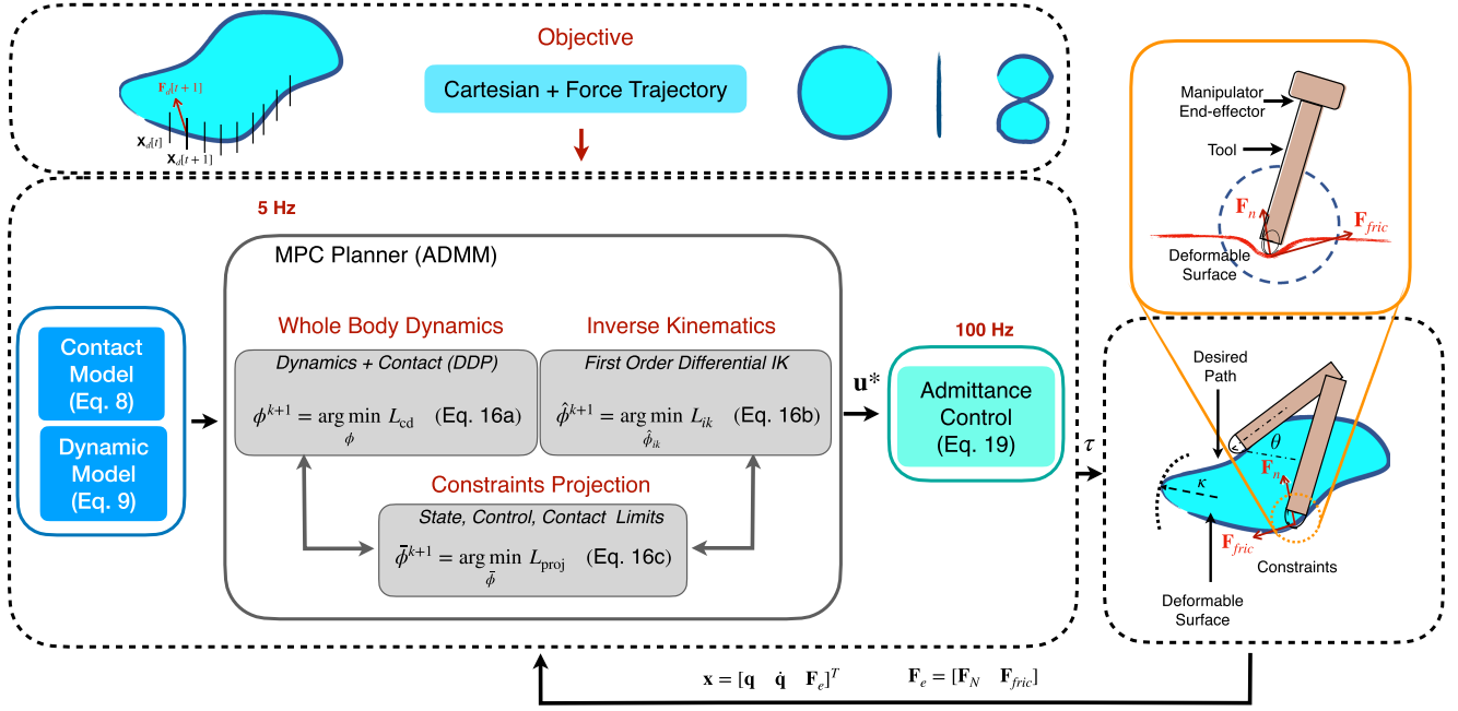
Fig. 4. Planning framework. The planner is composed of an ADMM-based solver executed in MPC fashion at 5 Hz. The ADMM solver contains three subblocks for optimization. Manipulator and contact dynamic models are used in the whole body dynamics block. Inverse kinematics block uses first-order differential kinematics to generate Cartesian trajectory. States are projected to satisfy the state and contact constraints in the projection block. The low-level FC, which is the admittance controller, is executed at 100 Hz. The desired Cartesian and force trajectory is tracked while obeying the constraints provided.
