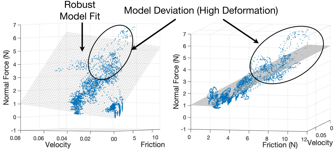
Fig. 8. Friction model validation and identification. \mu = 0.4512 , K_d = 13.1315 , and R-squared = 0.9103.
