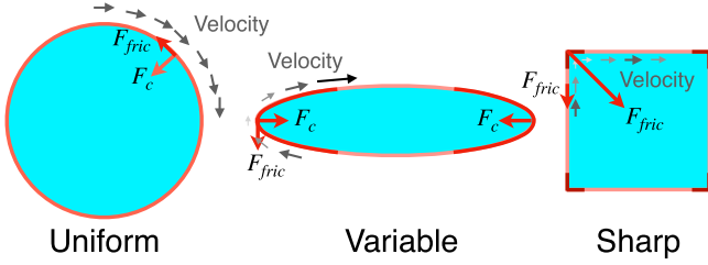
Fig. 3. Different Cartesian path geometries. At sharp corners of a Cartesian path, the robot needs to vary the velocity to compensate for centripetal and frictional force components caused through the contact.
