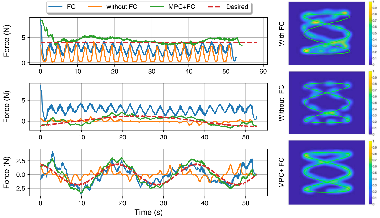
Fig. 10. Left: Normal and frictional forces with surface pulsations. Comparison of the activated FC (blue), inactivated force control (orange), and MPC and activated force control (green). Right: Normalized force and motion superimposed on a heat map. Note that motion pulsations of the experimental platform (see Fig. 6) cause the ripples observed in force profiles, for which the controller is attempting to compensate.
