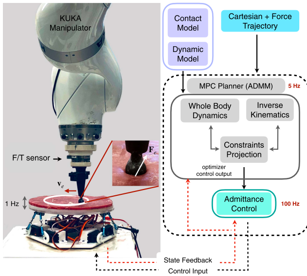
Fig. 1. KUKA manipulator experimentation setup, a manipulator performing a force-controlled motion task on a soft surface.
