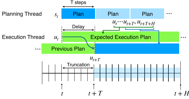
Fig. 5. MPC implementation. H , T , and s_t are the number of time steps for the horizon, time steps for the compute delay, and current state from the system, respectively. Computation takes T steps. During the time, execution thread keeps executing the previous plan. Once planning thread is finished, the current execution plan is updated; the time steps corresponding to delay is truncated.
