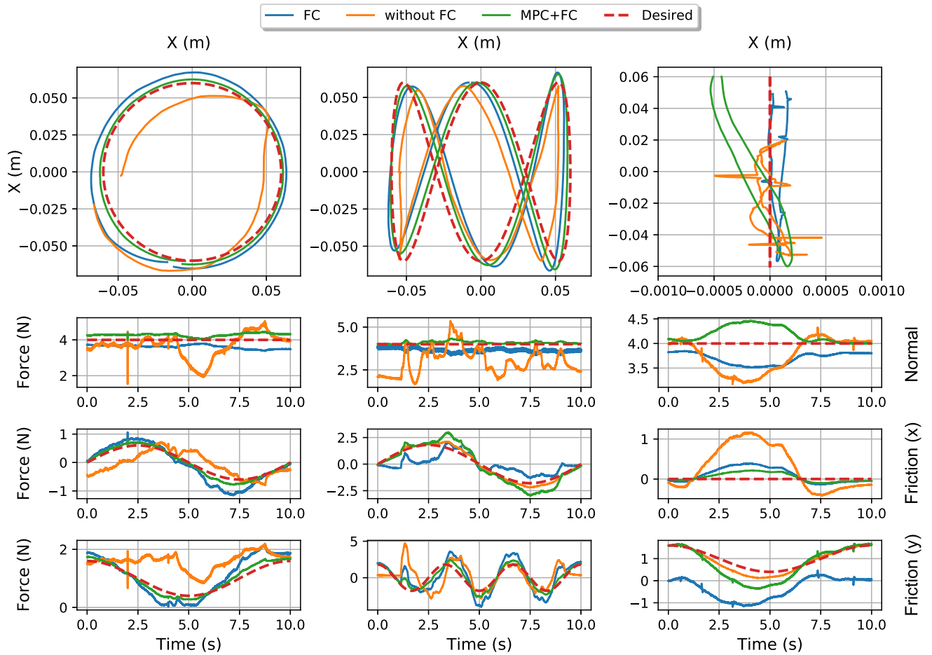
Fig. 9. Top row: Paths tracked by the end-effector versus commanded. Bottom Row: Comparison of ground truth of normal and frictional forces versus predicted by the model.
