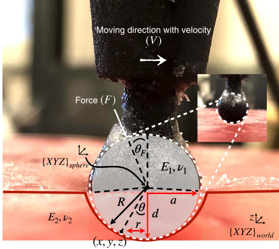
Fig. 2. Graphical illustration of the soft contact model between surface and the end-effector tool.
