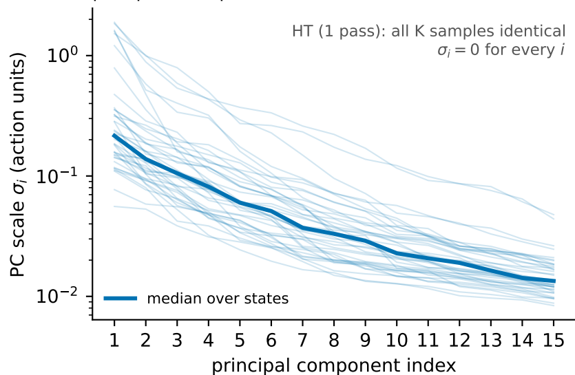
(a) GR1 flow (4 steps), 40 states sample spectrum per state; eff. rank median 3.1 of 232 dims
