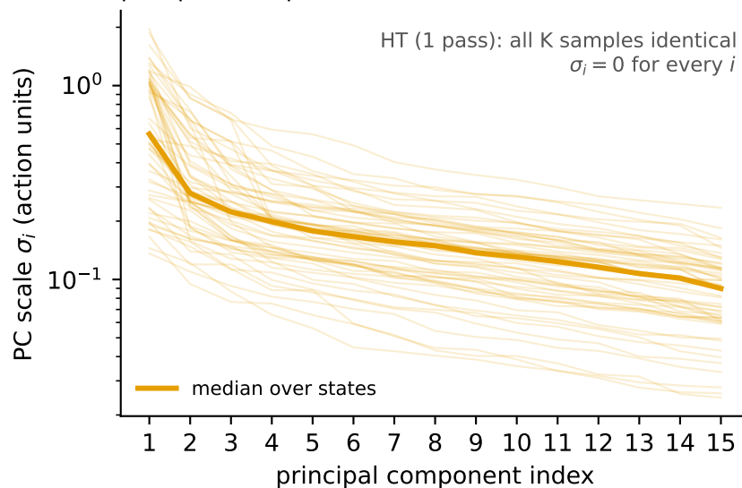
(b) \pi_{0.5} flow (10 steps), 60 states sample spectrum per state; eff. rank median 4.6 of 350 dims
