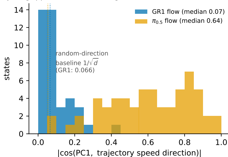
(d) is the dominant sampling axis the timing axis? \pi_{0.5} : yes (gripper-transition timing); GR1: no (median = random baseline)
