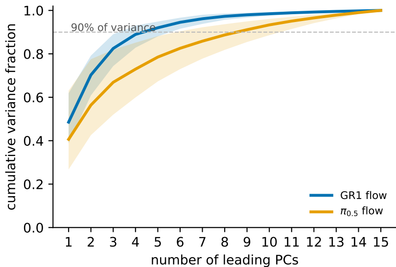
(c) variance captured by the leading PCs (median, IQR over states)
