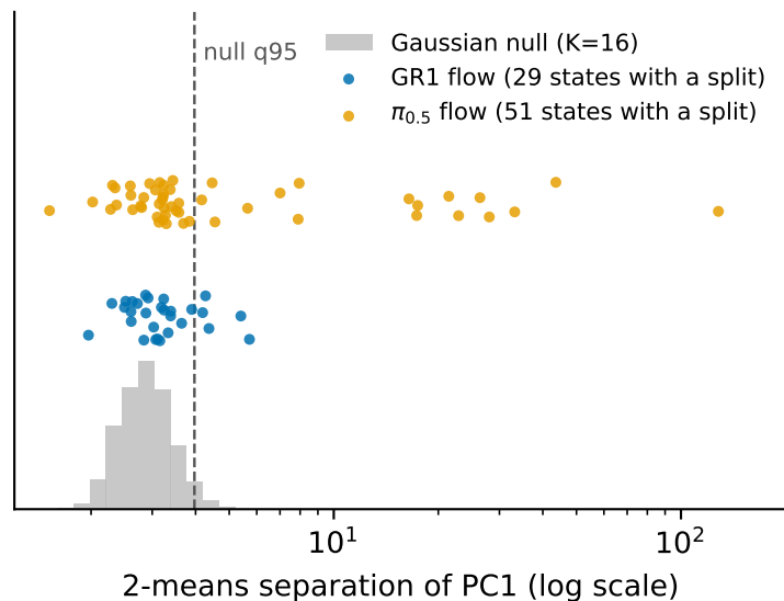
(c) separation at every probed state vs chance GR1 within chance; \pi_{0.5} has a tail
