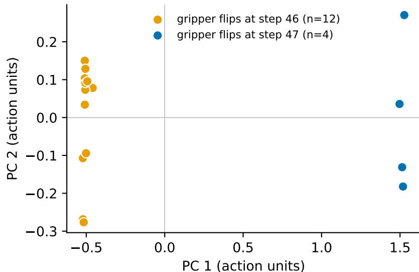
(a) PCA of 16 sampled chunks, one state looks bimodal: separation 128 (chance level 3.9)
