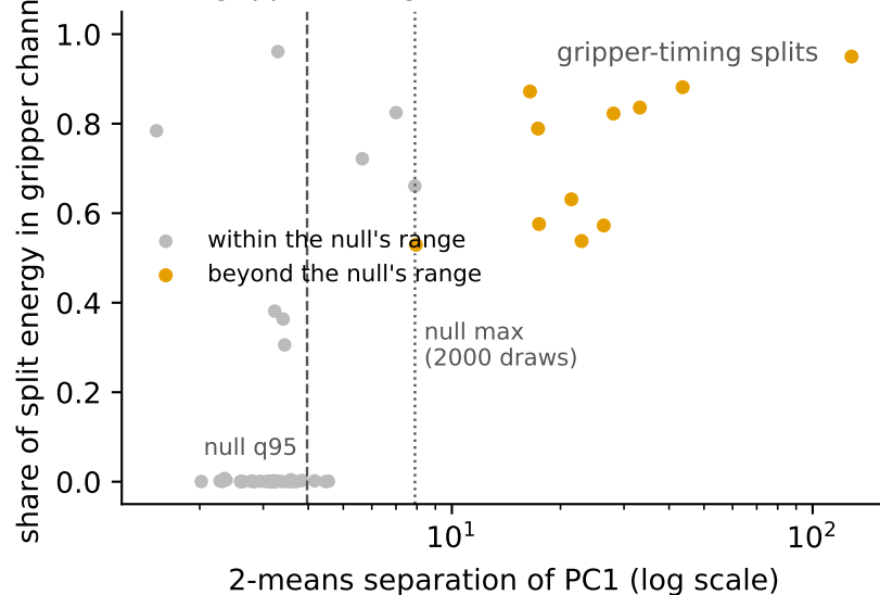
(d) \pi_{0.5} : every split beyond the null's range is gripper timing, not an alternative action
