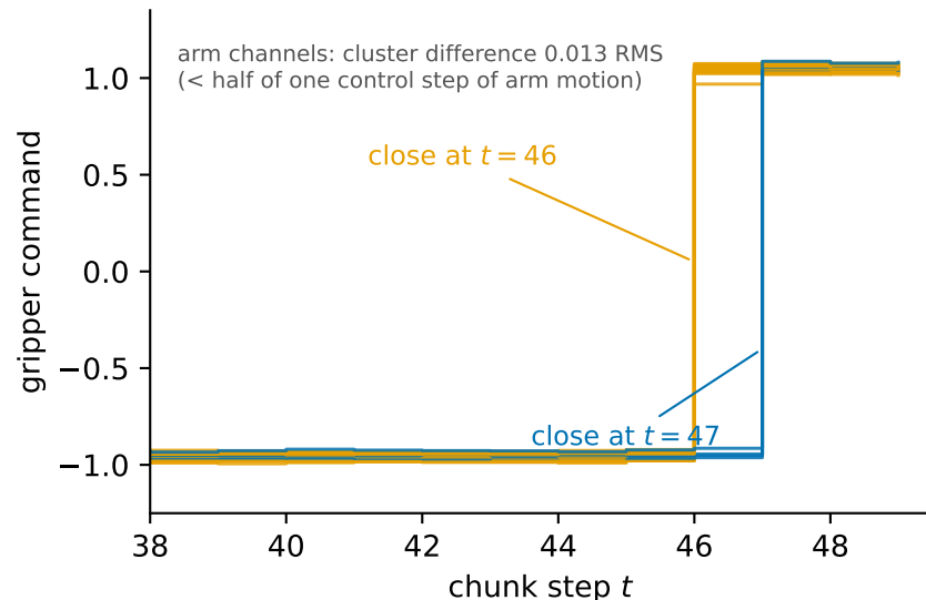
(b) same 16 samples, gripper channel identical action, one step apart in time
