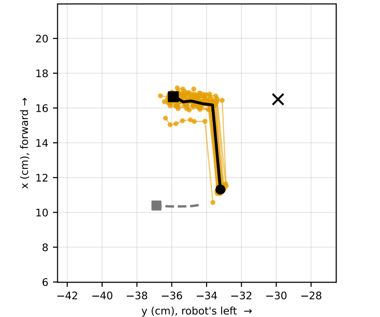
GR1 flow, typical state (ep 53, step 239) scatter around mean path: mean 0.4 / max 1.6 cm; at chunk end 0.5 cm
