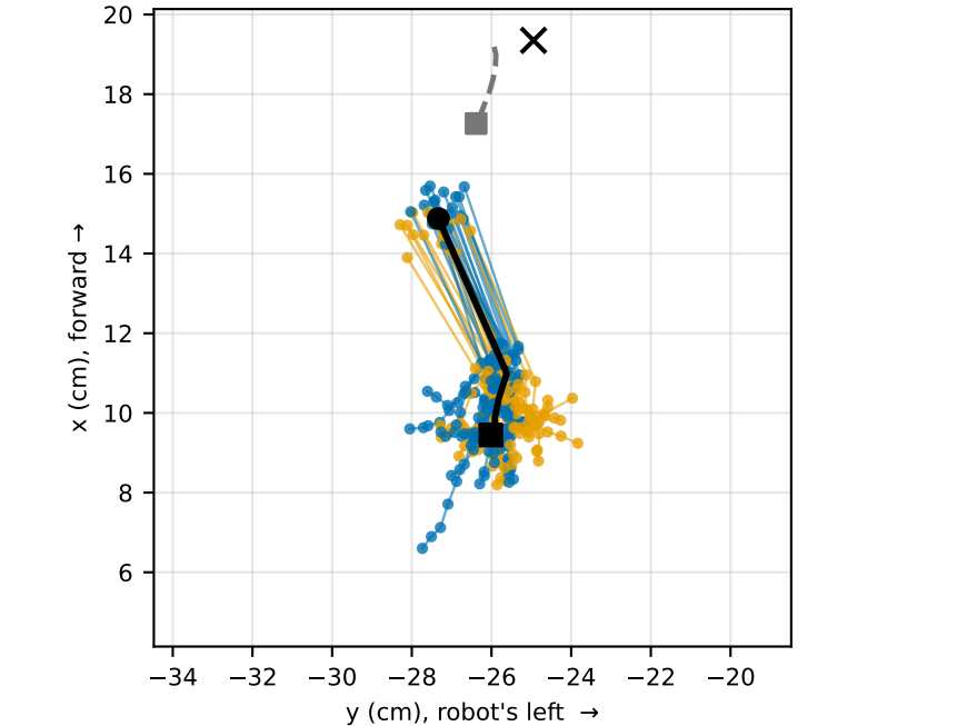
GR1 flow, most separated state in 3000 (ep 801, step 1, K=32) scatter around mean path: mean 1.2 / max 3.7 cm; at chunk end 1.9 cm
