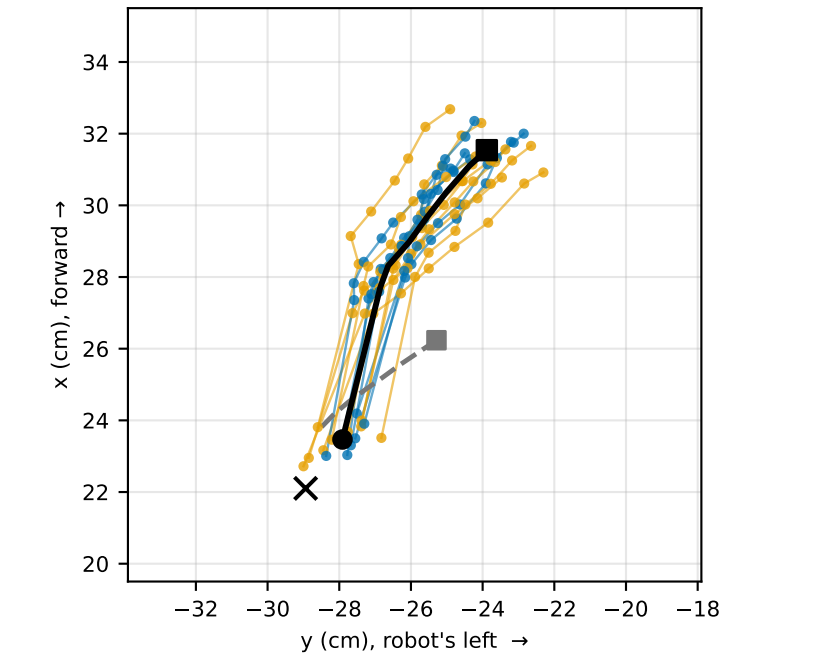
GR1 flow, widest state (ep 706, step 39) scatter around mean path: mean 0.9 / max 1.8 cm; at chunk end 0.9 cm
