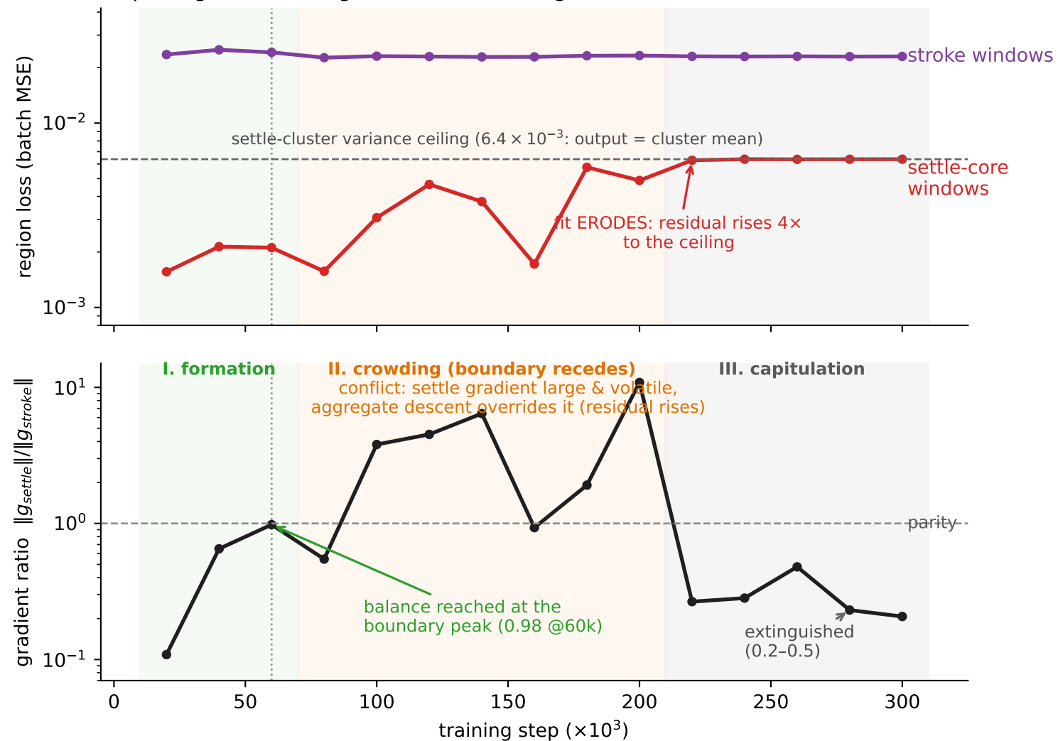
L2: per-region loss and gradient over training (128 settle-core / 128 stroke windows)
