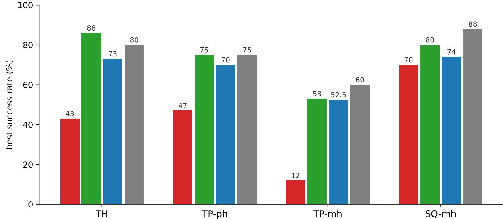
Human-data tasks: best SR by loss family
