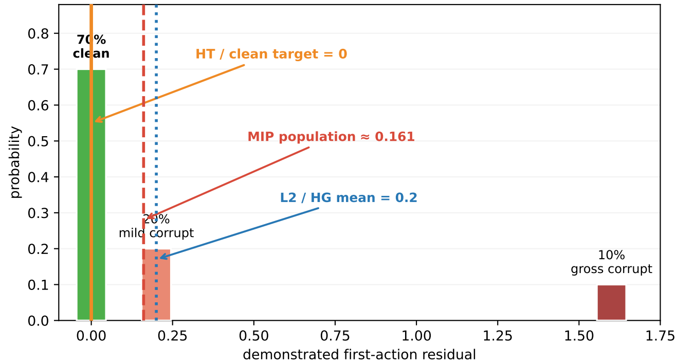
A Put the label mean on a corrupt branch
