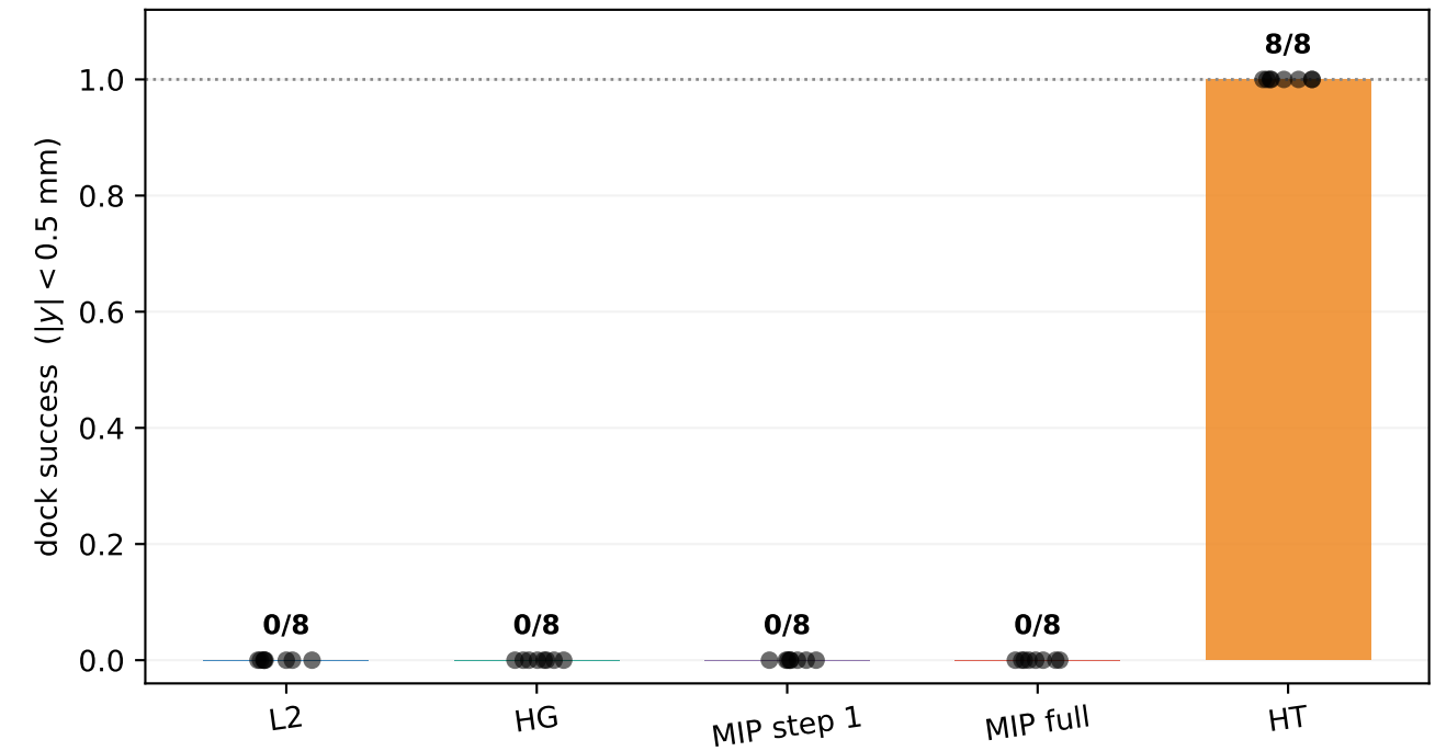
B HT is the only successful estimator
