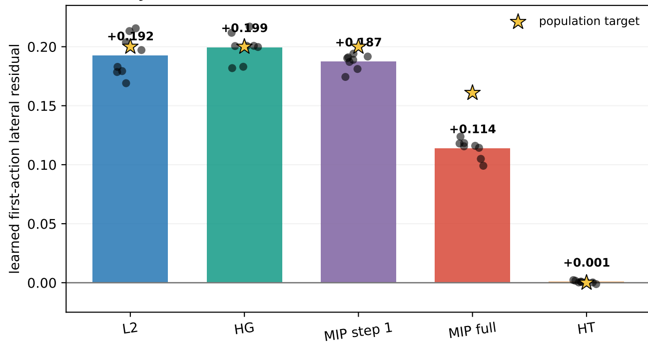
C HT rejects both contaminant scales and recovers zero
