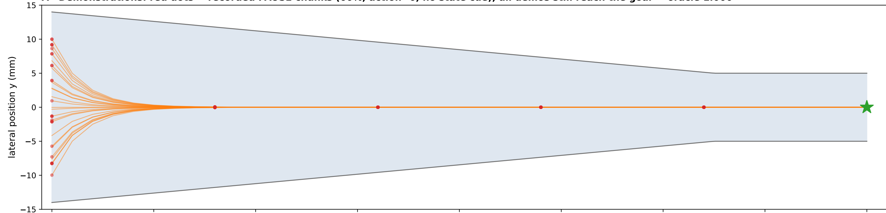
B Trained policies: mean family and diffusion travel to the goal; HT nu=0.5 commits to the pause mode and PARKS (dots at start)
