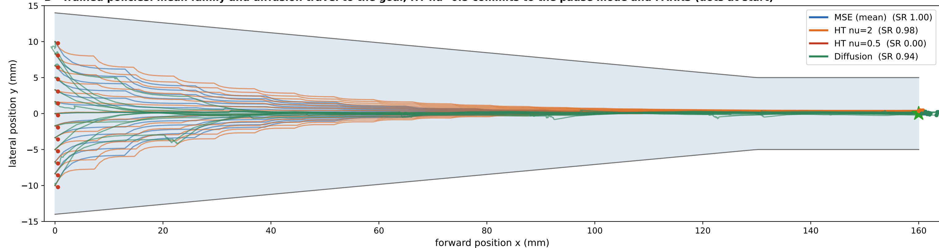
B Trained policies: mean family and diffusion travel to the goal; HT nu=0.5 commits to the pause mode and PARKS (dots at start)
