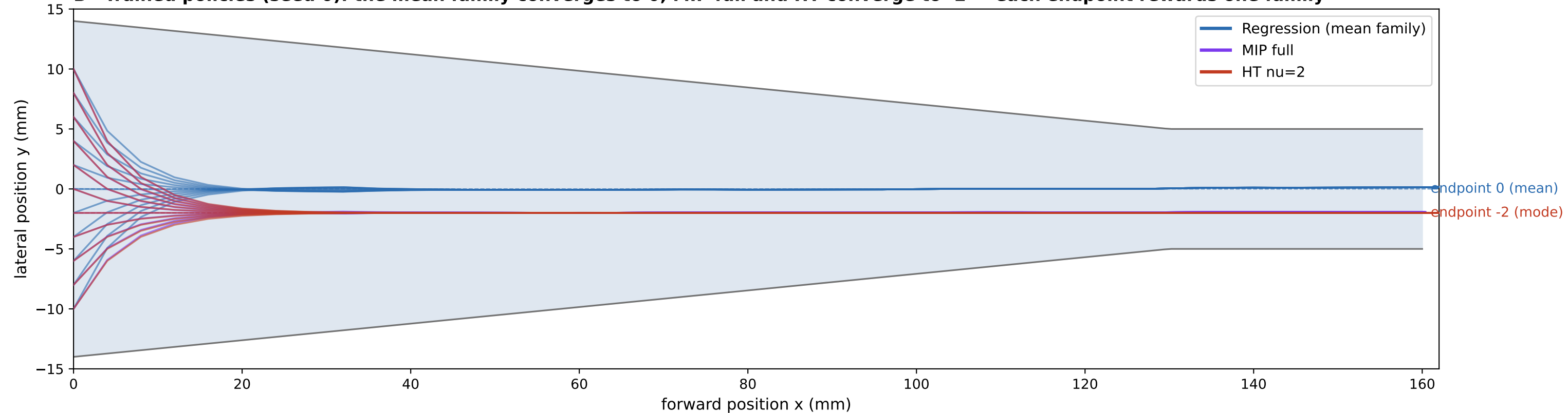
B Trained policies (seed 0): the mean family converges to 0; MIP full and HT converge to -2 — each endpoint rewards one family
