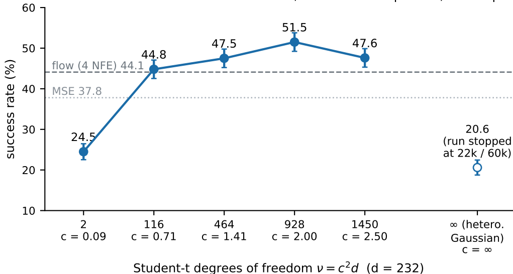
GR00T N1.7 on RoboCasa GR1: HT head, 24 tasks x 20 episodes, 60k steps
