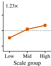
Chi-UNet Tool-Hang
