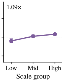
Chi-UNet Transport
