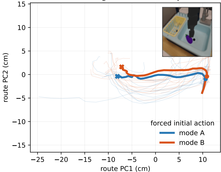
b basket: strongest confirmed split
