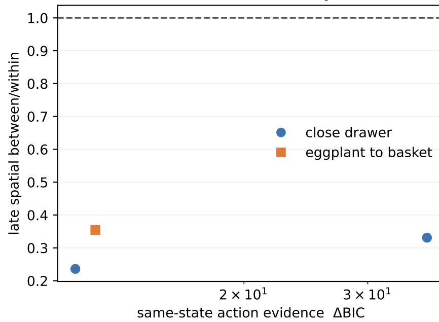
e action evidence vs. late separation
