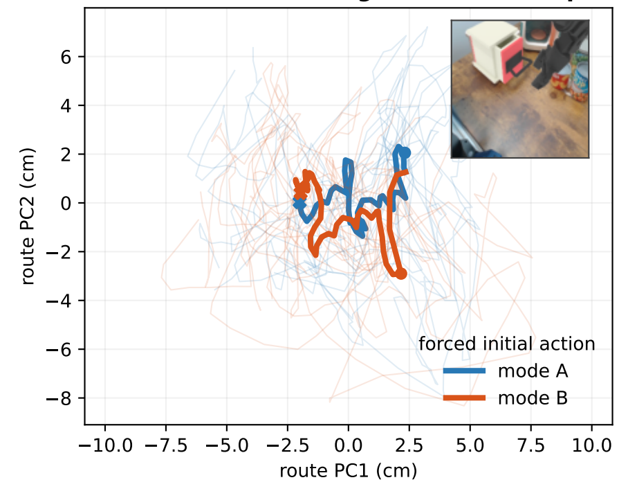
d mode-conditioned spatial separation over time
