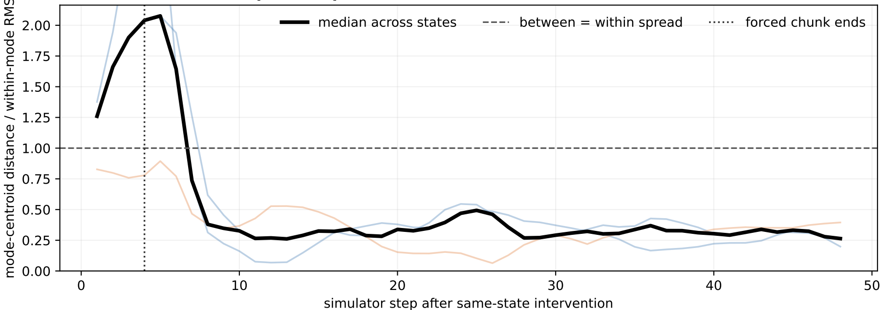
d mode-conditioned spatial separation over time
