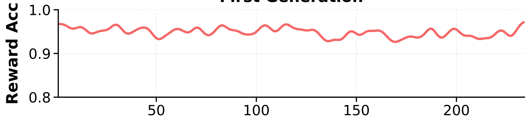
Self-verification
