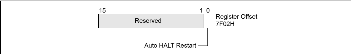
Figure 32-3. Auto HALT Restart Field
