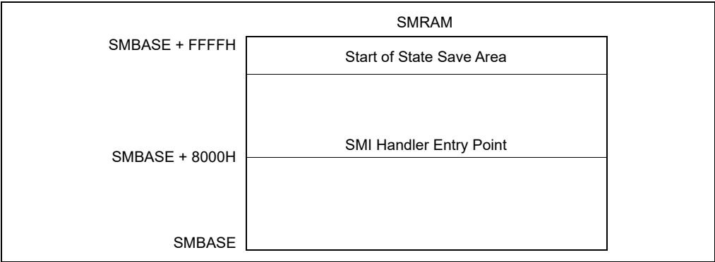
Figure 32-1. SMRAM Usage
