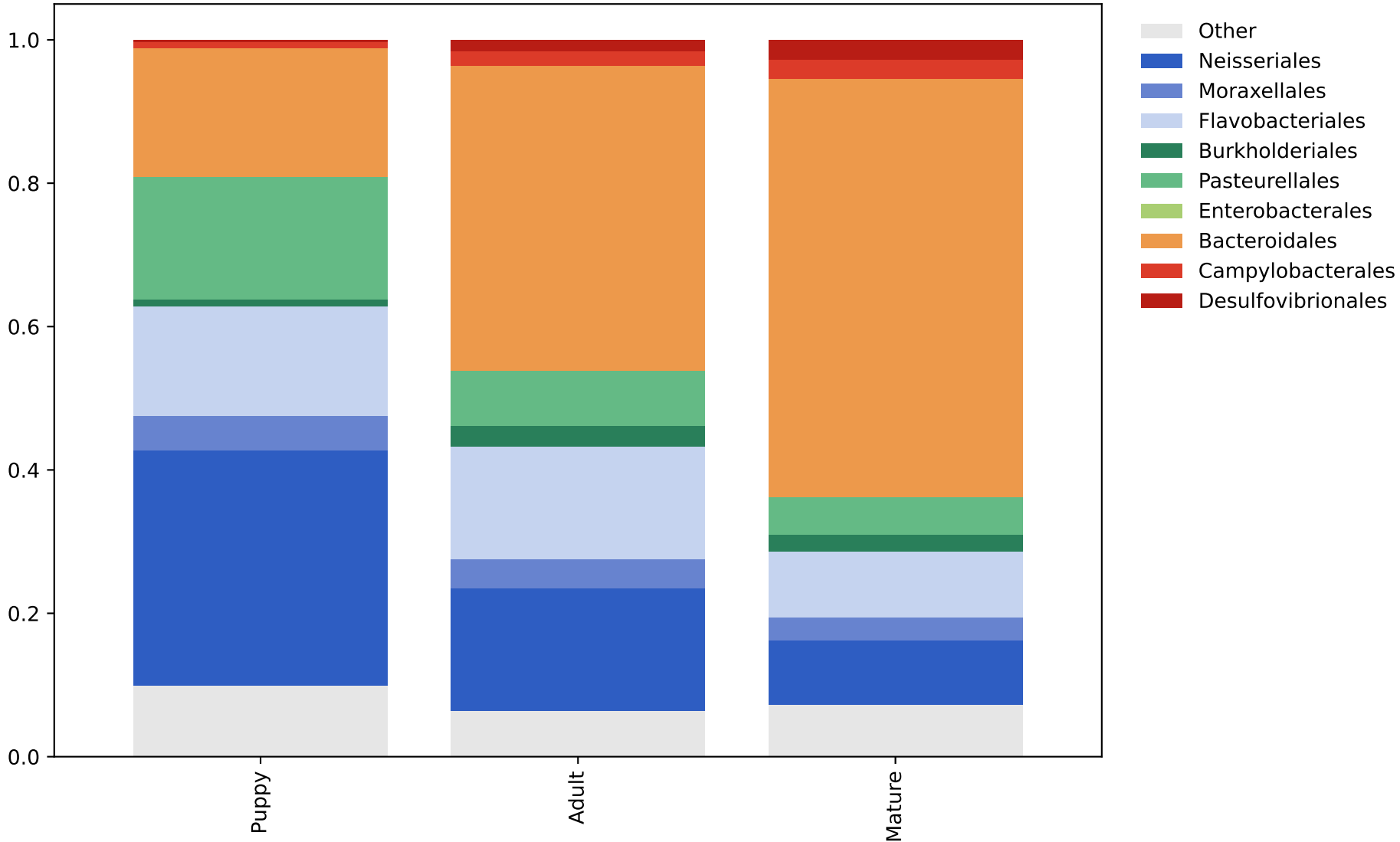
Mean relative abundance among classified orders
