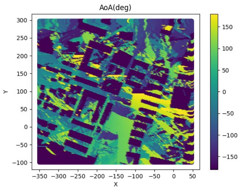
AoA map
