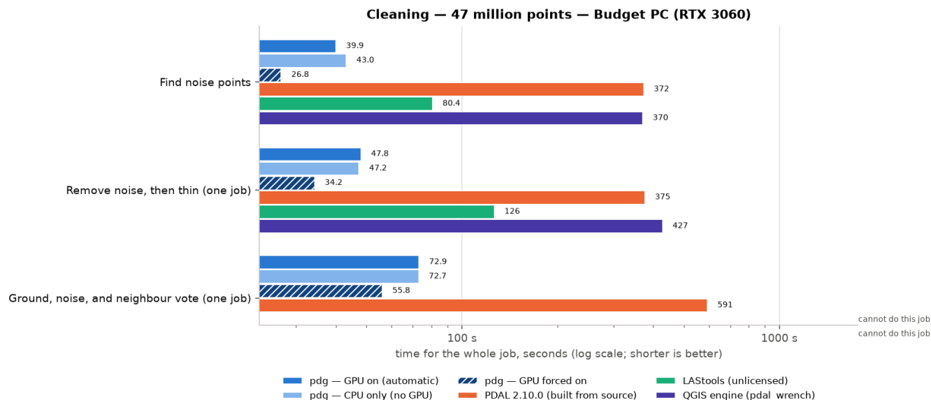
Cleaning: median time in seconds, 47 million points, Budget PC (RTX 3060).
