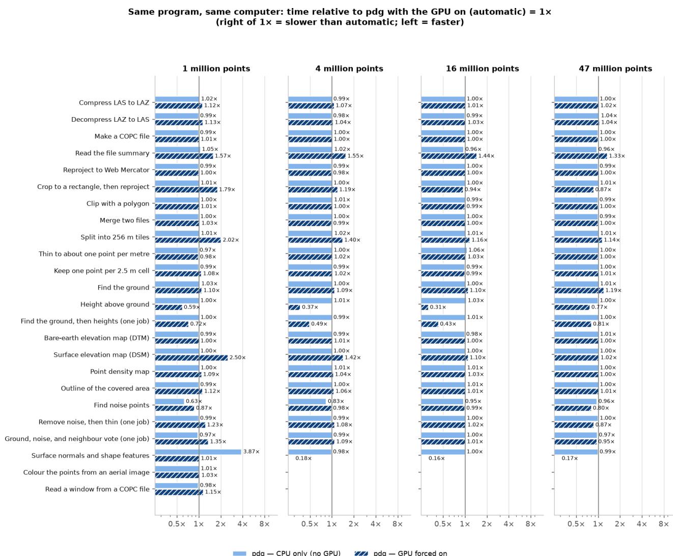
Figure. pdg CPU-only and GPU-forced time divided by pdg automatic time, per job and file size, workstation (RTX 4090).
