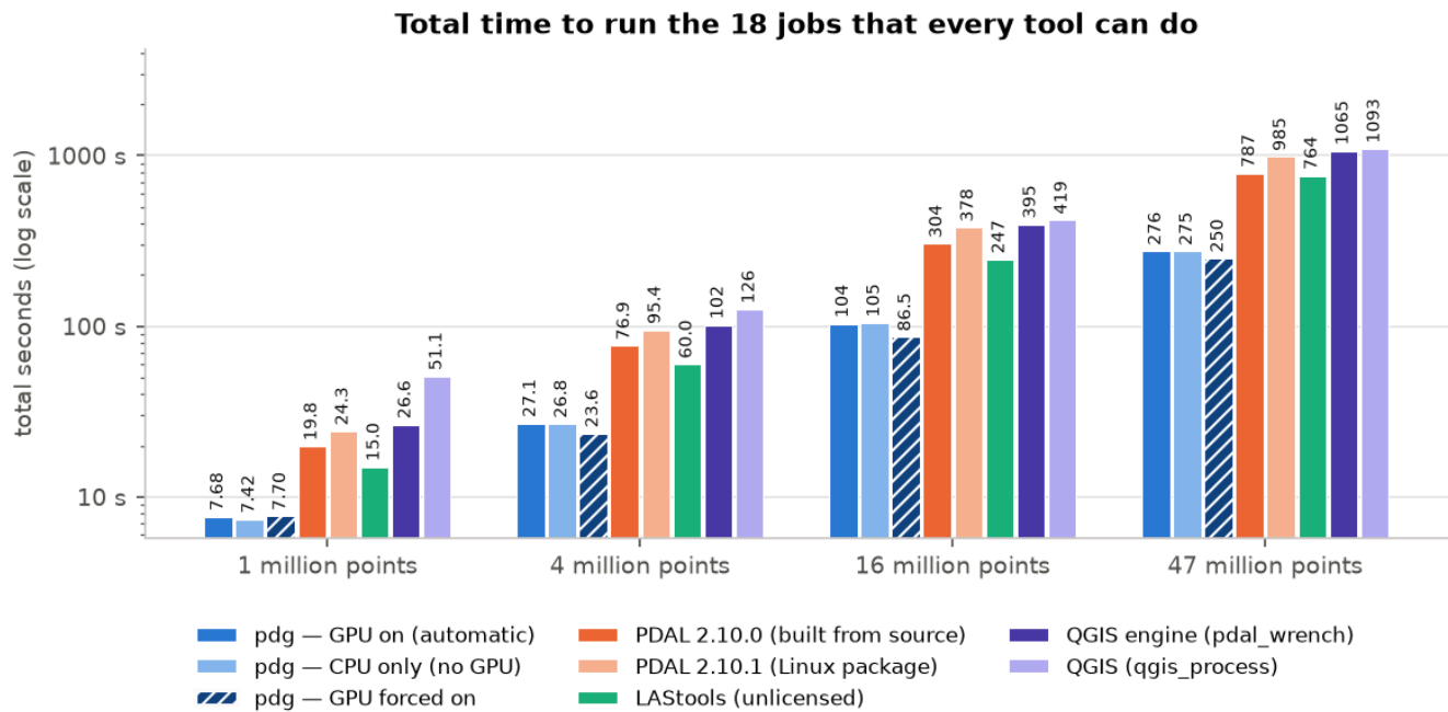
Figure. Total time to run, one after another, the jobs that every tool can do at every size ().
