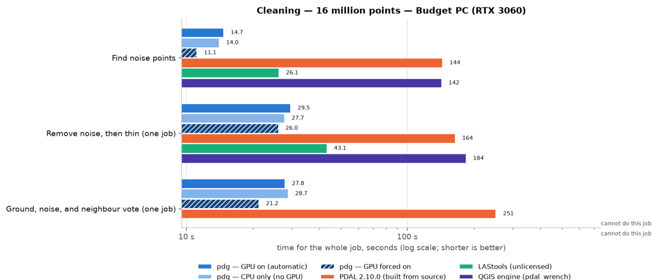
Cleaning: median time in seconds, 16 million points, Budget PC (RTX 3060).
