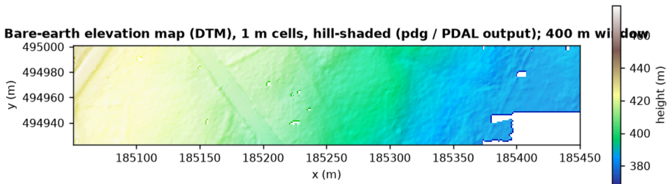
Figure. "Bare-earth elevation map (DTM)" from pdg / PDAL, hill-shaded.
