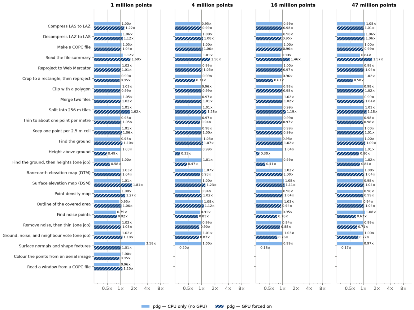
Figure. pdg CPU-only and GPU-forced time relative to automatic, Budget PC (RTX 3060).
