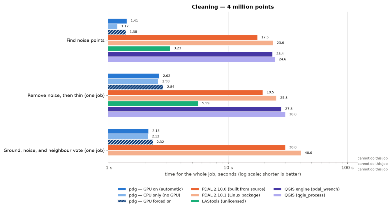
Cleaning: median time in seconds, 4 million points, workstation.
