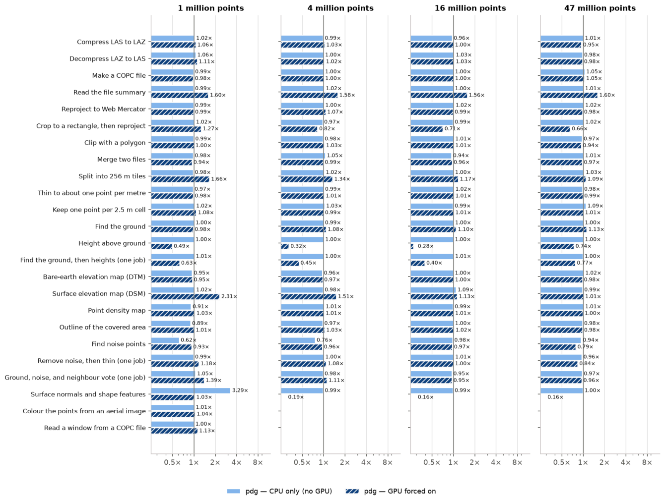
Figure. pdg CPU-only and GPU-forced time relative to automatic, Cloud server (A100).
