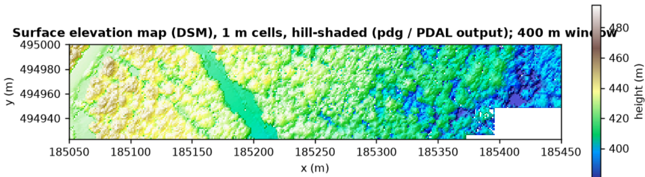
Figure. "Surface elevation map (DSM)": highest first return per 1 m cell (pdg / PDAL output).
