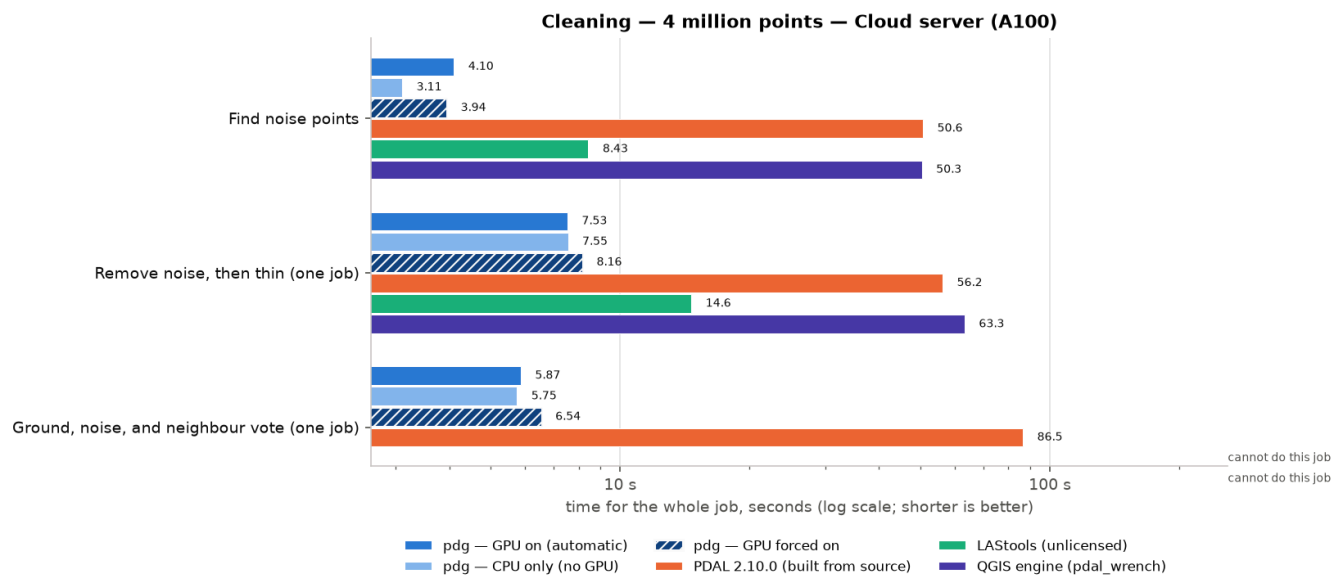
Cleaning: median time in seconds, 4 million points, Cloud server (A100).
