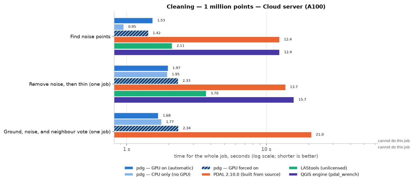
Cleaning: median time in seconds, 1 million points, Cloud server (A100).
