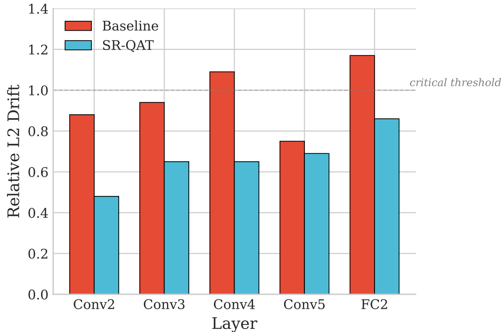
(a) Layer-wise Activation Drift
