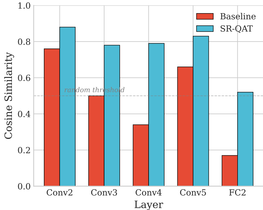
(b) Layer-wise Activation Similarity
