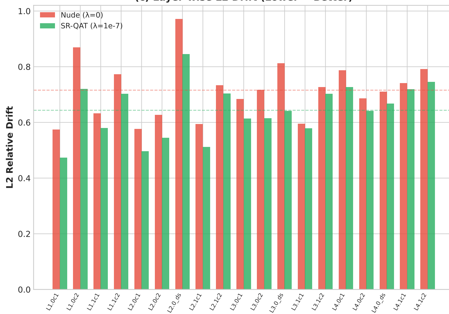
(c) Layer-wise L2 Drift (Lower = Better)
