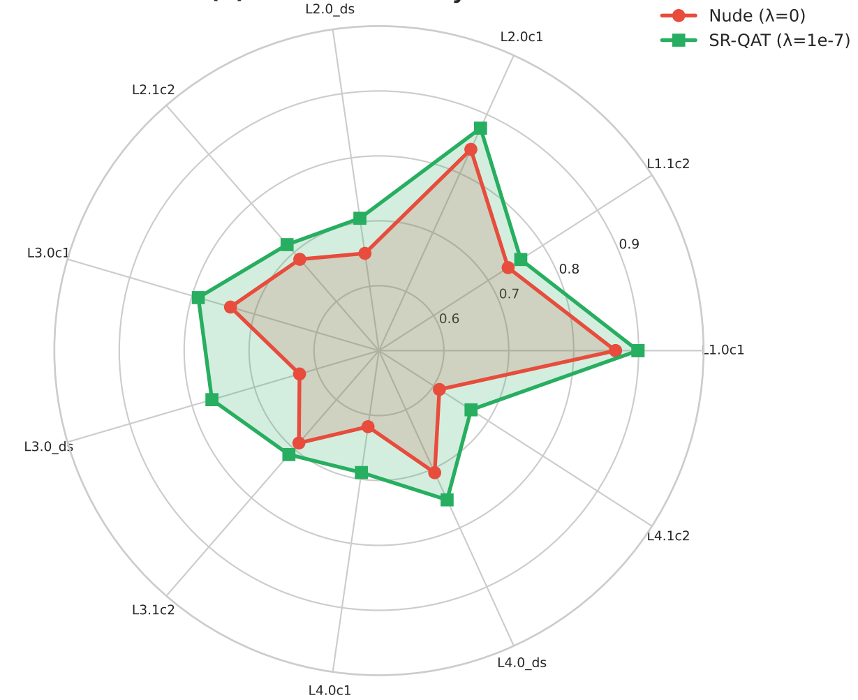
(b) Cosine Similarity Radar
